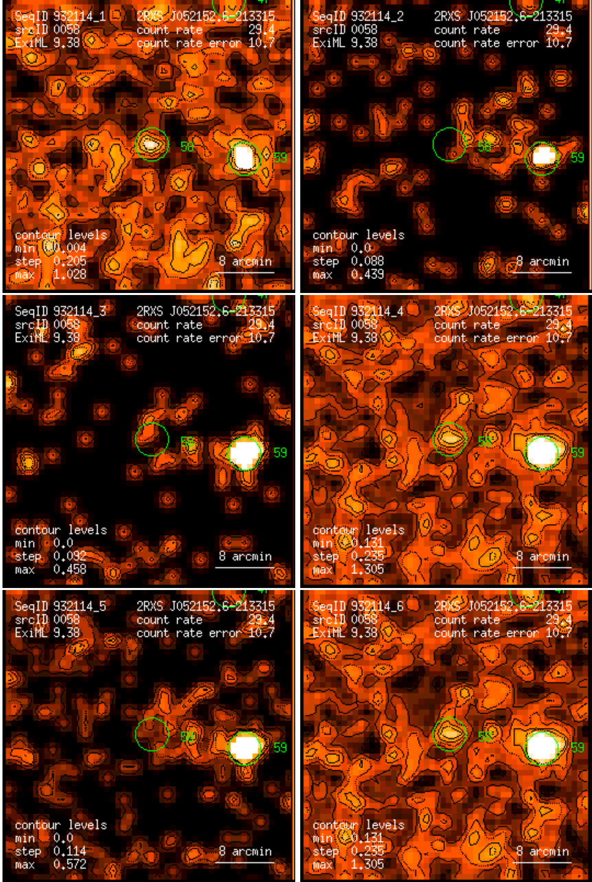
Figure 58: RASS 932114: detection 0058: band rate images, Gaussian filter: (1) PSPC channels 11 – 41, (2) 52 – 90, (3) 91 – 201, (4) 11 – 235, (5) 52 – 201, (6) 11 – 201. Broad band rates in counts/ks. Band rate contour levels in counts/ks/arcmin 2 .
