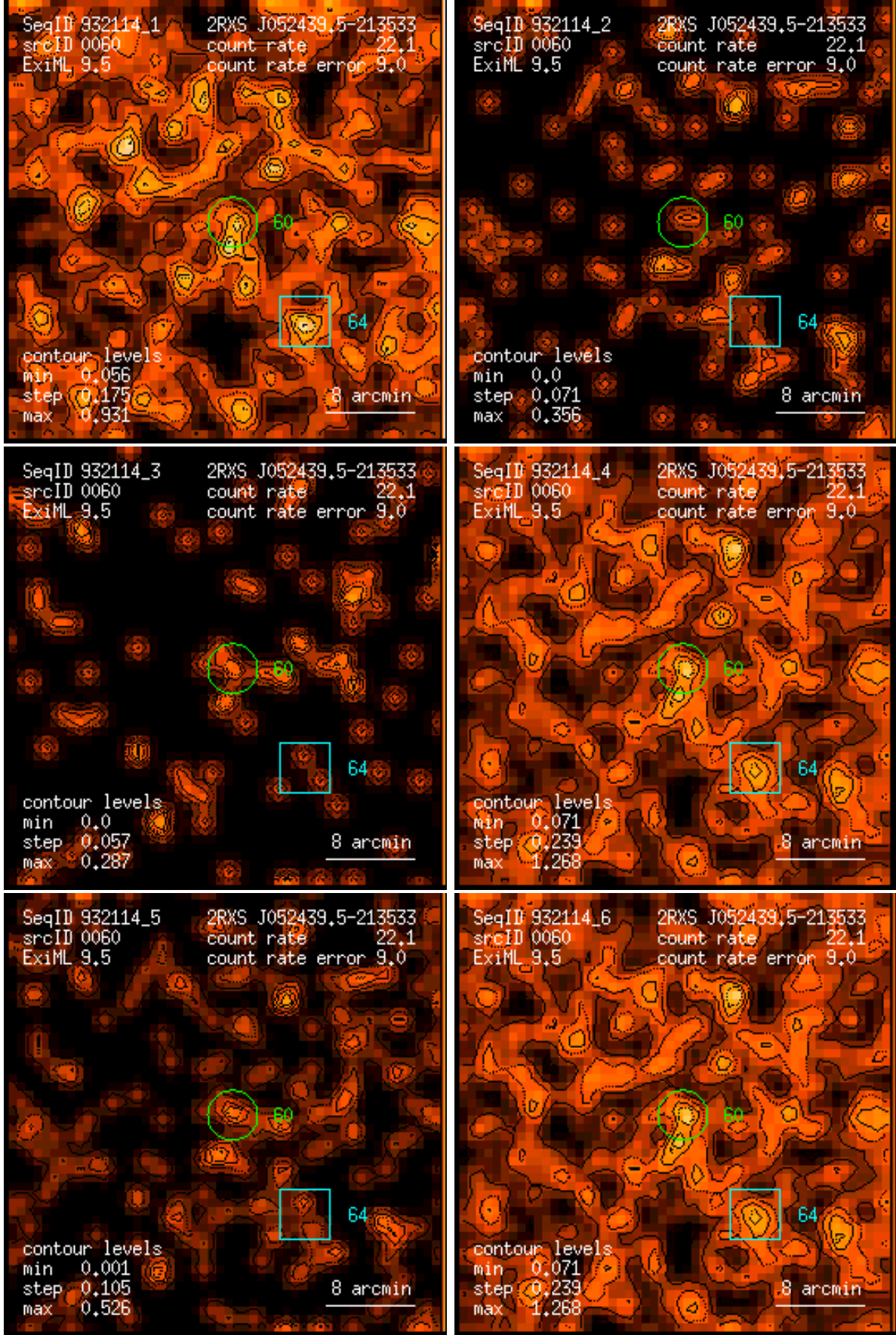
Figure 60: RASS 932114: detection 0060: band rate images, Gaussian filter: (1) PSPC channels 11 – 41, (2) 52 – 90, (3) 91 – 201, (4) 11 – 235, (5) 52 – 201, (6) 11 – 201. Broad band rates in counts/ks. Band rate contour levels in counts/ks/arcmin 2 .
