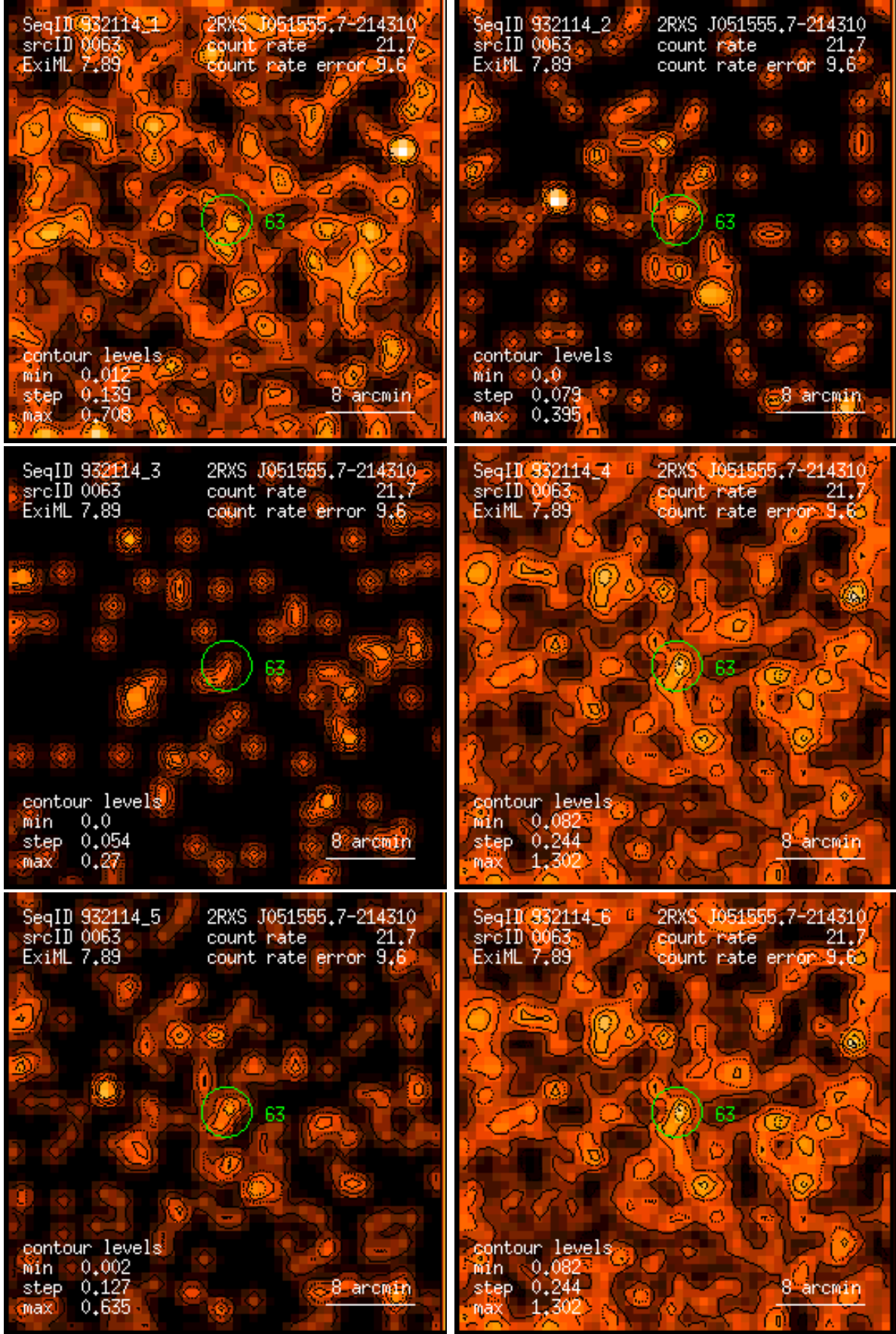
Figure 63: RASS 932114: detection 0063: band rate images, Gaussian filter: (1) PSPC channels 11 – 41, (2) 52 – 90, (3) 91 – 201, (4) 11 – 235, (5) 52 – 201, (6) 11 – 201. Broad band rates in counts/ks. Band rate contour levels in counts/ks/arcmin 2 .
