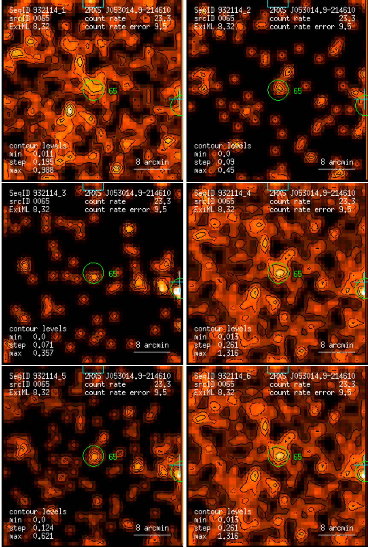
Figure 65: RASS 932114: detection 0065: band rate images, Gaussian filter: (1) PSPC channels 11 – 41, (2) 52 – 90, (3) 91 – 201, (4) 11 – 235, (5) 52 – 201, (6) 11 – 201. Broad band rates in counts/ks. Band rate contour levels in counts/ks/arcmin 2 .
