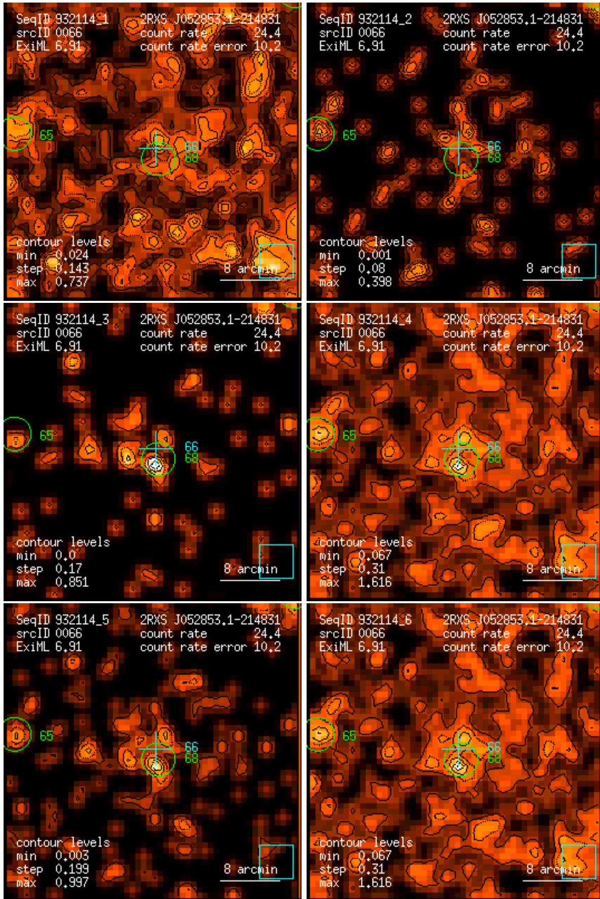
Figure 66: RASS 932114: detection 0066: band rate images, Gaussian filter: (1) PSPC channels 11 – 41, (2) 52 – 90, (3) 91 – 201, (4) 11 – 235, (5) 52 – 201, (6) 11 – 201. Broad band rates in counts/ks. Band rate contour levels in counts/ks/arcmin 2 .
