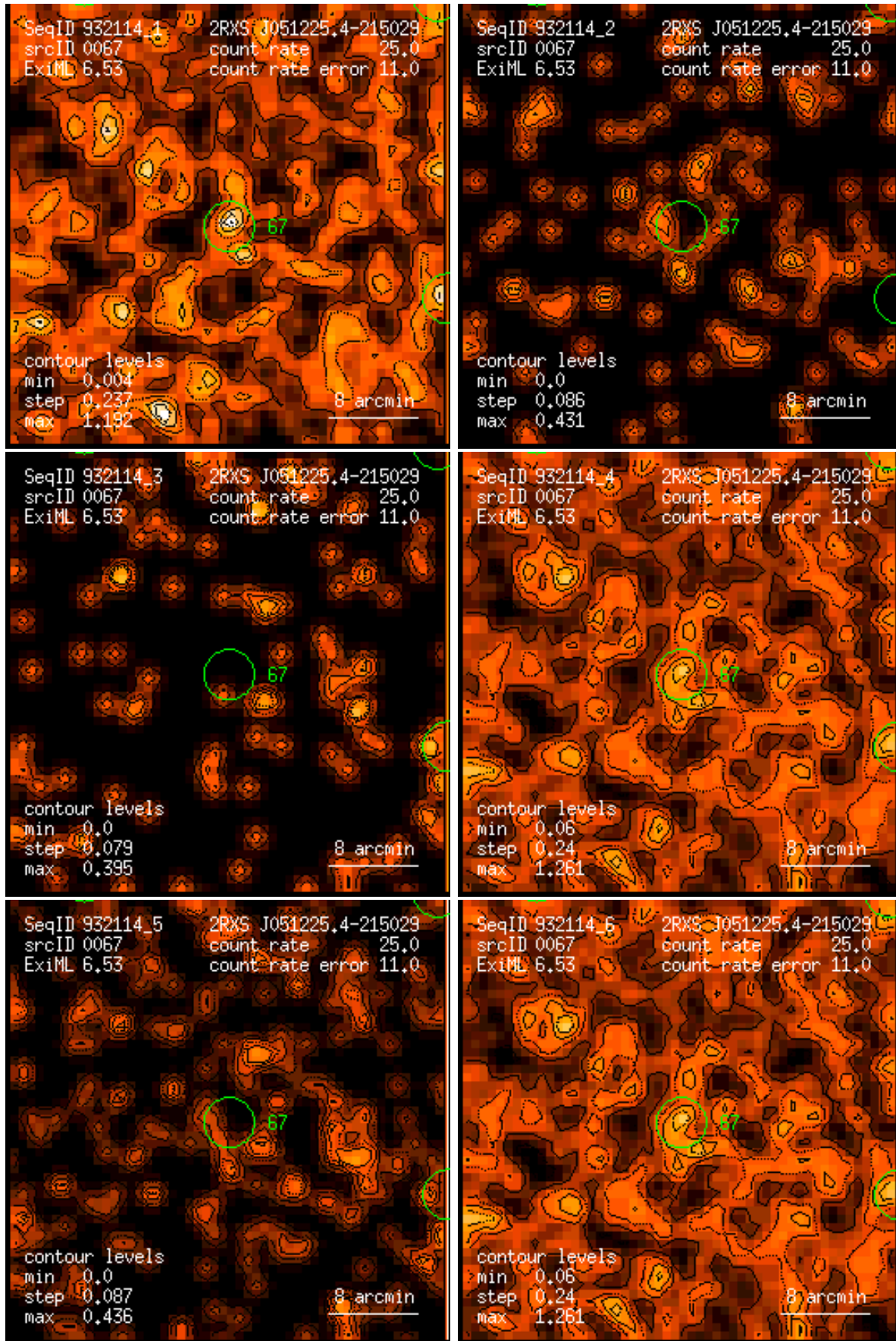
Figure 67: RASS 932114: detection 0067: band rate images, Gaussian filter: (1) PSPC channels 11 – 41, (2) 52 – 90, (3) 91 – 201, (4) 11 – 235, (5) 52 – 201, (6) 11 – 201. Broad band rates in counts/ks. Band rate contour levels in counts/ks/arcmin 2 .
