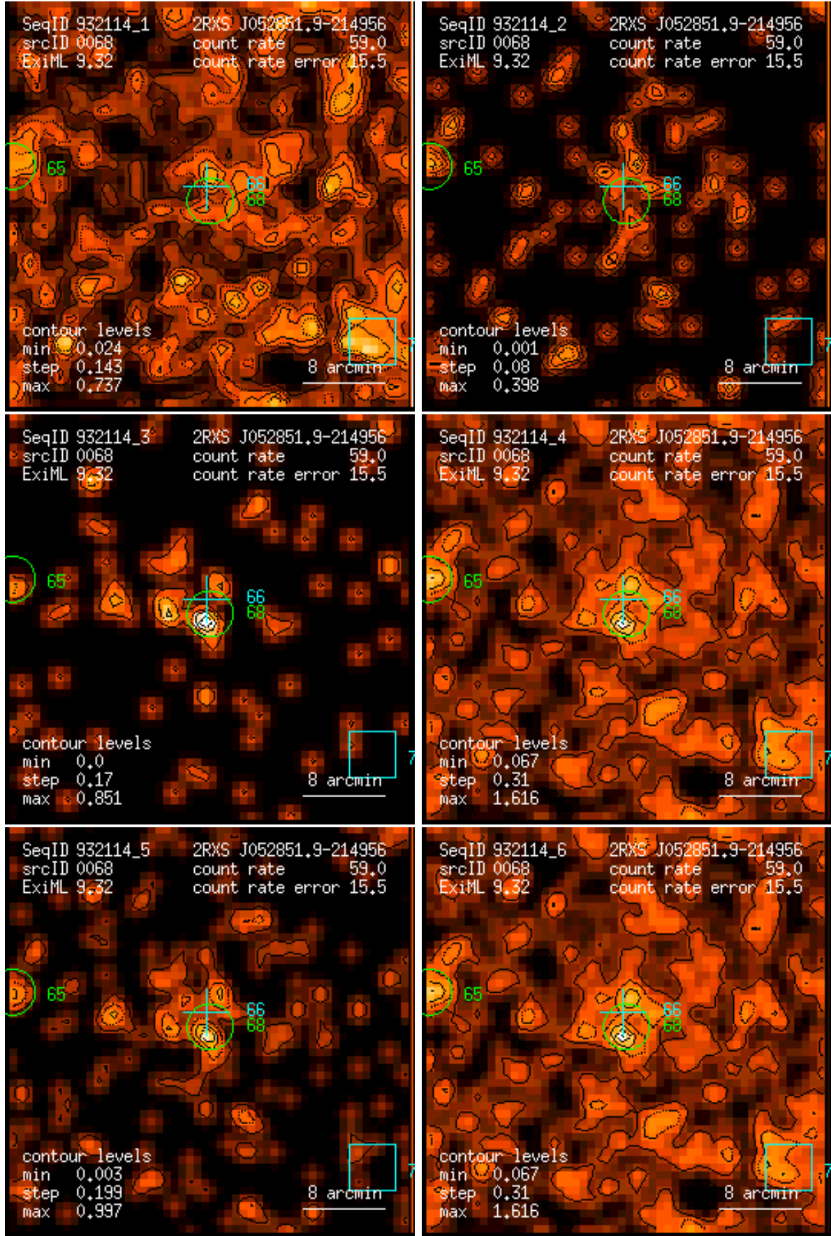
Figure 68: RASS 932114: detection 0068: band rate images, Gaussian filter: (1) PSPC channels 11 – 41, (2) 52 – 90, (3) 91 – 201, (4) 11 – 235, (5) 52 – 201, (6) 11 – 201. Broad band rates in counts/ks. Band rate contour levels in counts/ks/arcmin 2 .
