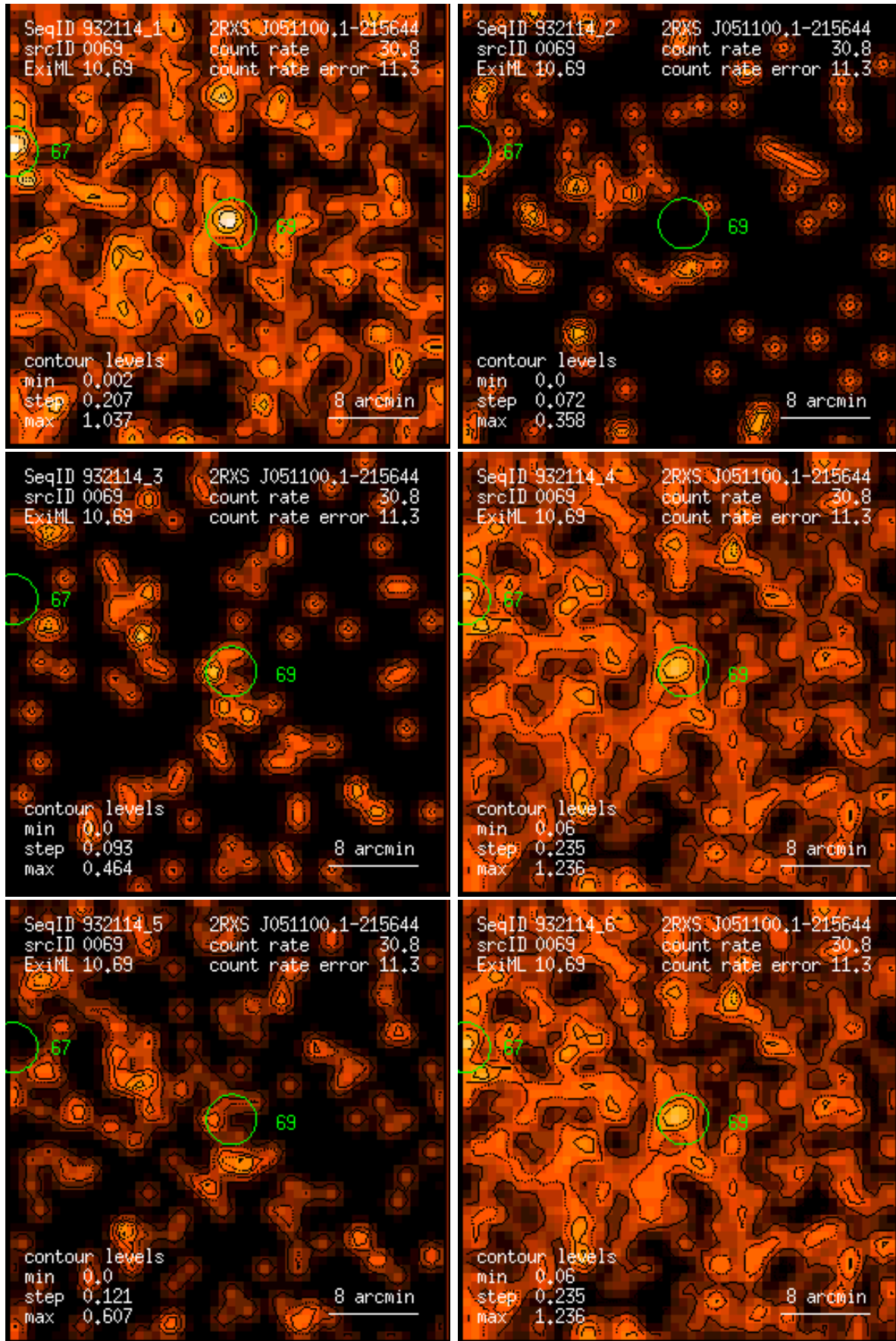
Figure 69: RASS 932114: detection 0069: band rate images, Gaussian filter: (1) PSPC channels 11 – 41, (2) 52 – 90, (3) 91 – 201, (4) 11 – 235, (5) 52 – 201, (6) 11 – 201. Broad band rates in counts/ks. Band rate contour levels in counts/ks/arcmin 2 .
