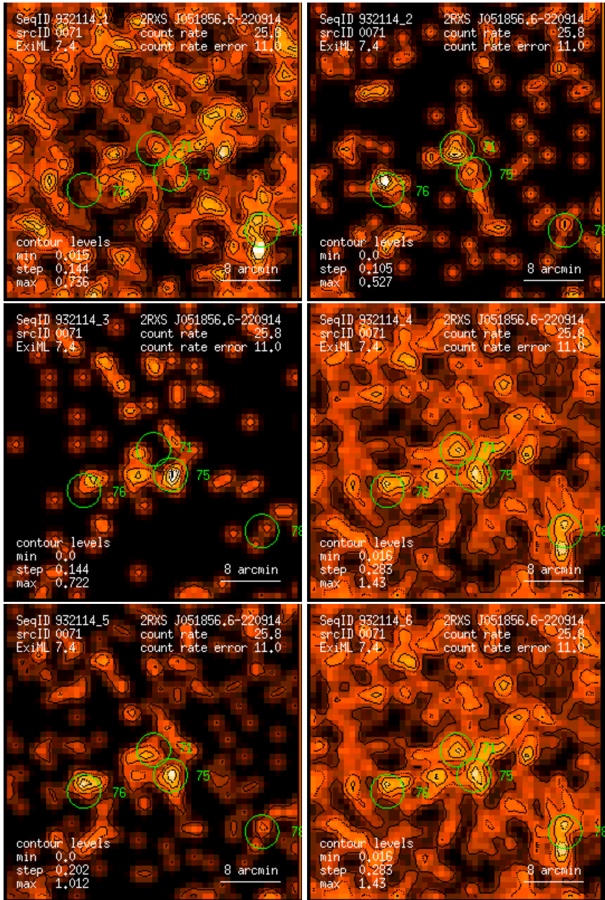
Figure 71: RASS 932114: detection 0071: band rate images, Gaussian filter: (1) PSPC channels 11 – 41, (2) 52 – 90, (3) 91 – 201, (4) 11 – 235, (5) 52 – 201, (6) 11 – 201. Broad band rates in counts/ks. Band rate contour levels in counts/ks/arcmin 2 .
