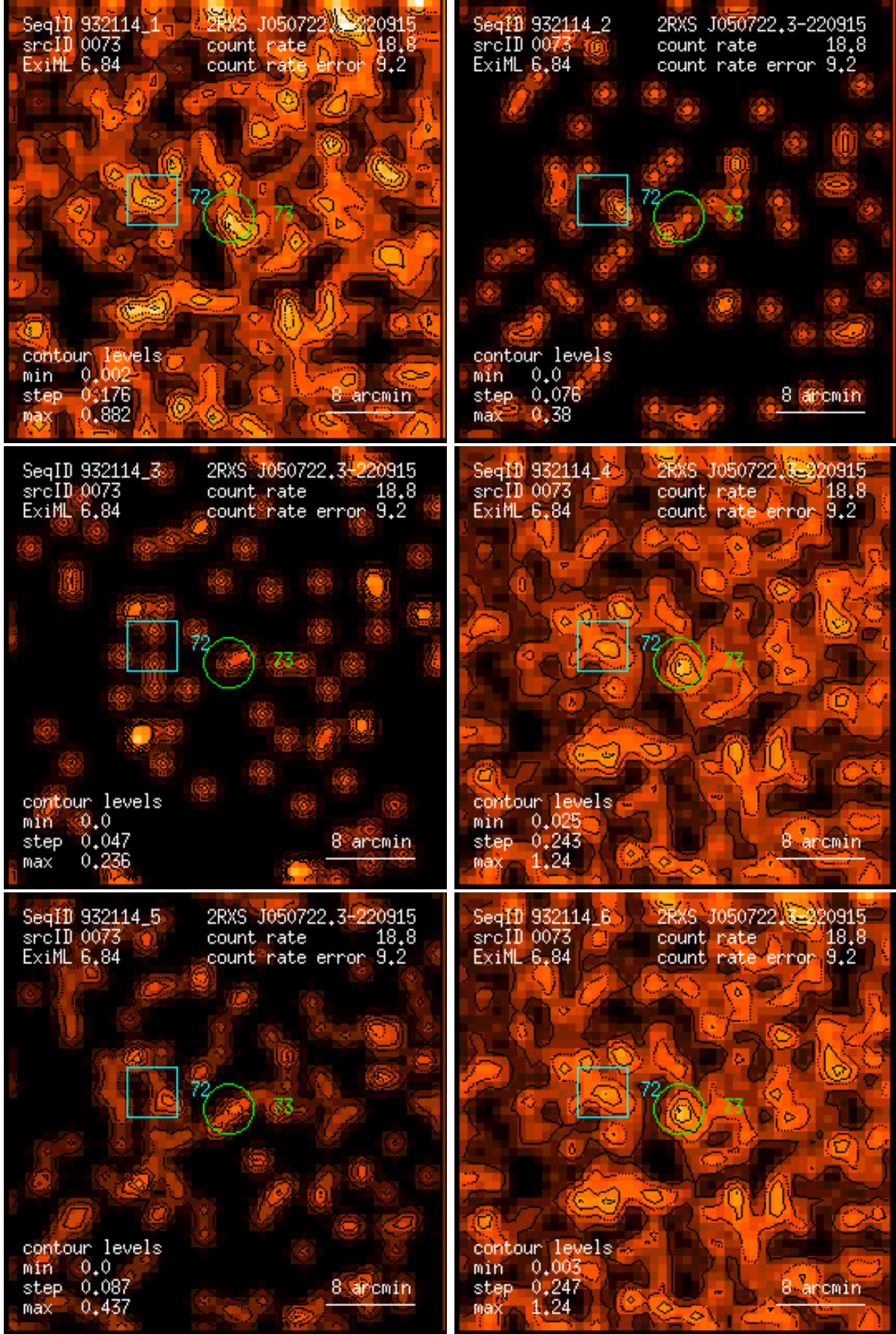
Figure 73: RASS 932114: detection 0073: band rate images, Gaussian filter: (1) PSPC channels 11 – 41, (2) 52 – 90, (3) 91 – 201, (4) 11 – 235, (5) 52 – 201, (6) 11 – 201. Broad band rates in counts/ks. Band rate contour levels in counts/ks/arcmin 2 .
