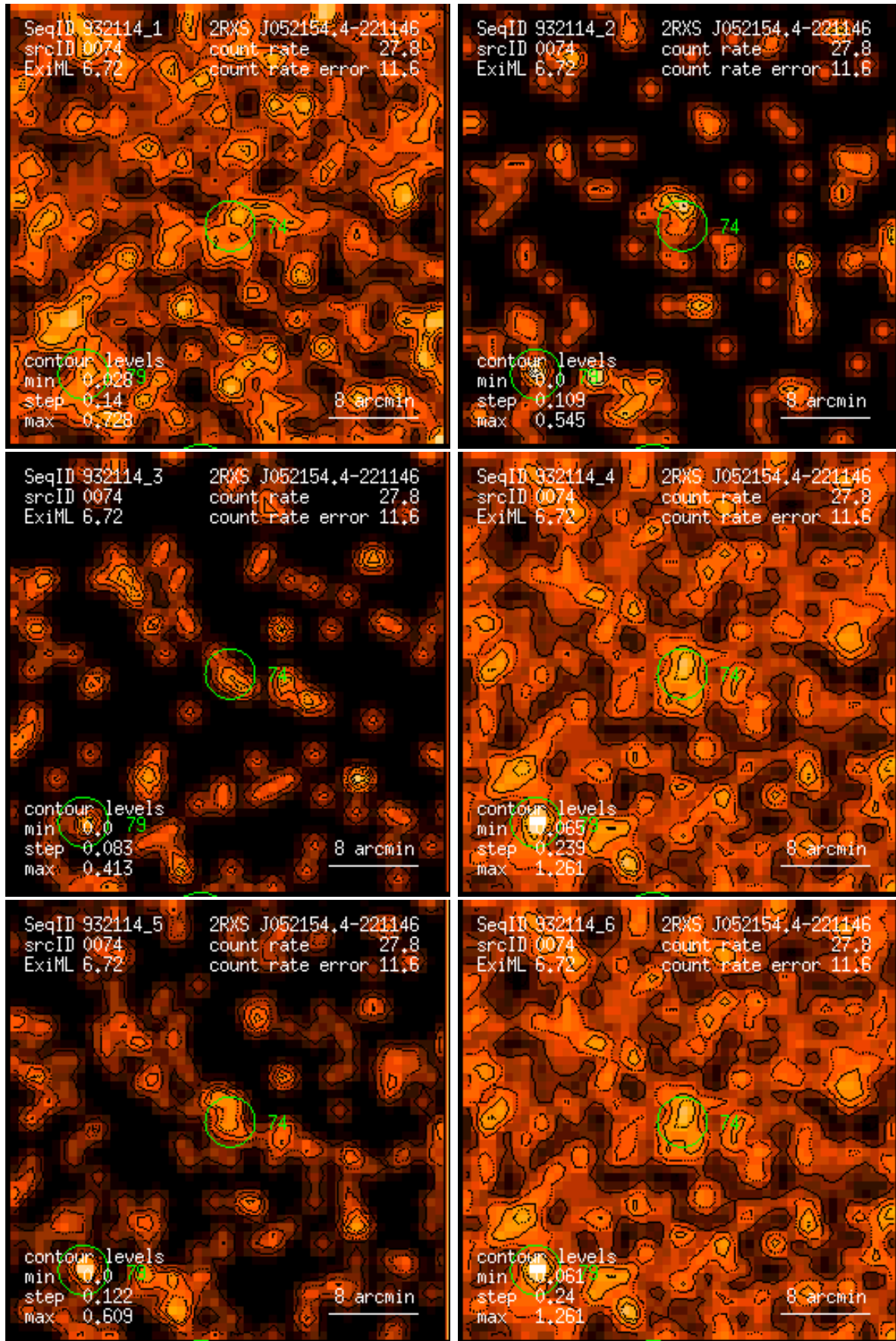
Figure 74: RASS 932114: detection 0074: band rate images, Gaussian filter: (1) PSPC channels 11 – 41, (2) 52 – 90, (3) 91 – 201, (4) 11 – 235, (5) 52 – 201, (6) 11 – 201. Broad band rates in counts/ks. Band rate contour levels in counts/ks/arcmin 2 .
