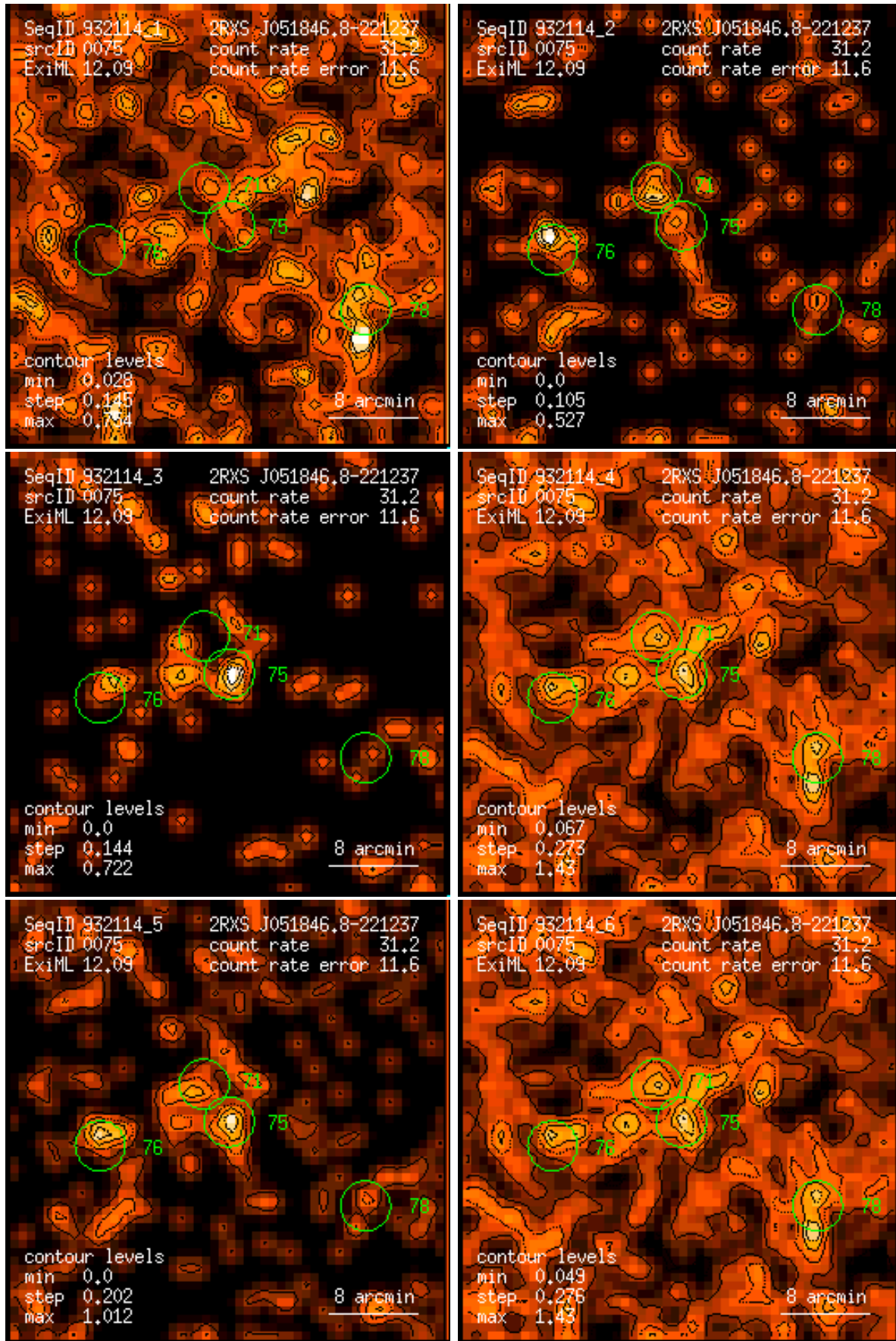
Figure 75: RASS 932114: detection 0075: band rate images, Gaussian filter: (1) PSPC channels 11 – 41, (2) 52 – 90, (3) 91 – 201, (4) 11 – 235, (5) 52 – 201, (6) 11 – 201. Broad band rates in counts/ks. Band rate contour levels in counts/ks/arcmin 2 .
