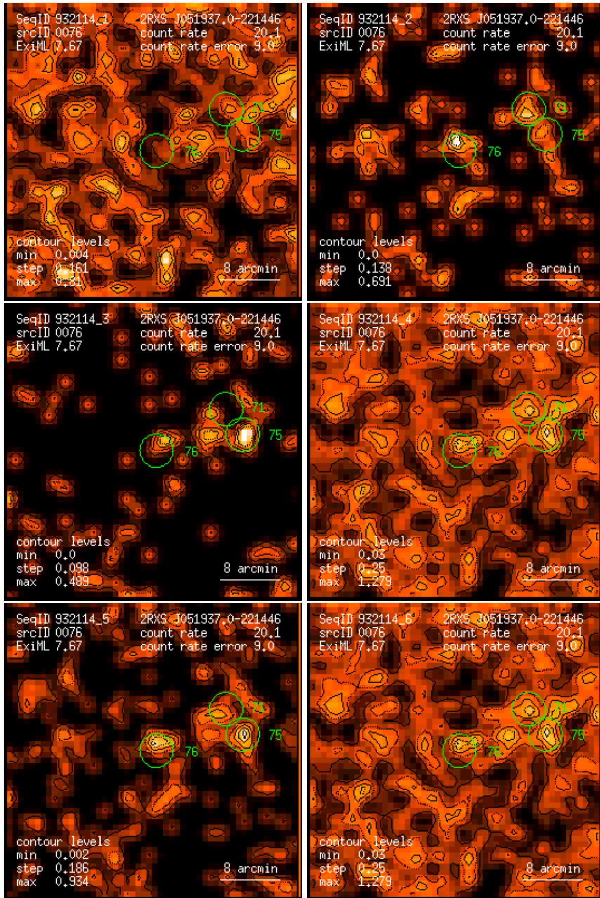
Figure 76: RASS 932114: detection 0076: band rate images, Gaussian filter: (1) PSPC channels 11 – 41, (2) 52 – 90, (3) 91 – 201, (4) 11 – 235, (5) 52 – 201, (6) 11 – 201. Broad band rates in counts/ks. Band rate contour levels in counts/ks/arcmin 2 .
