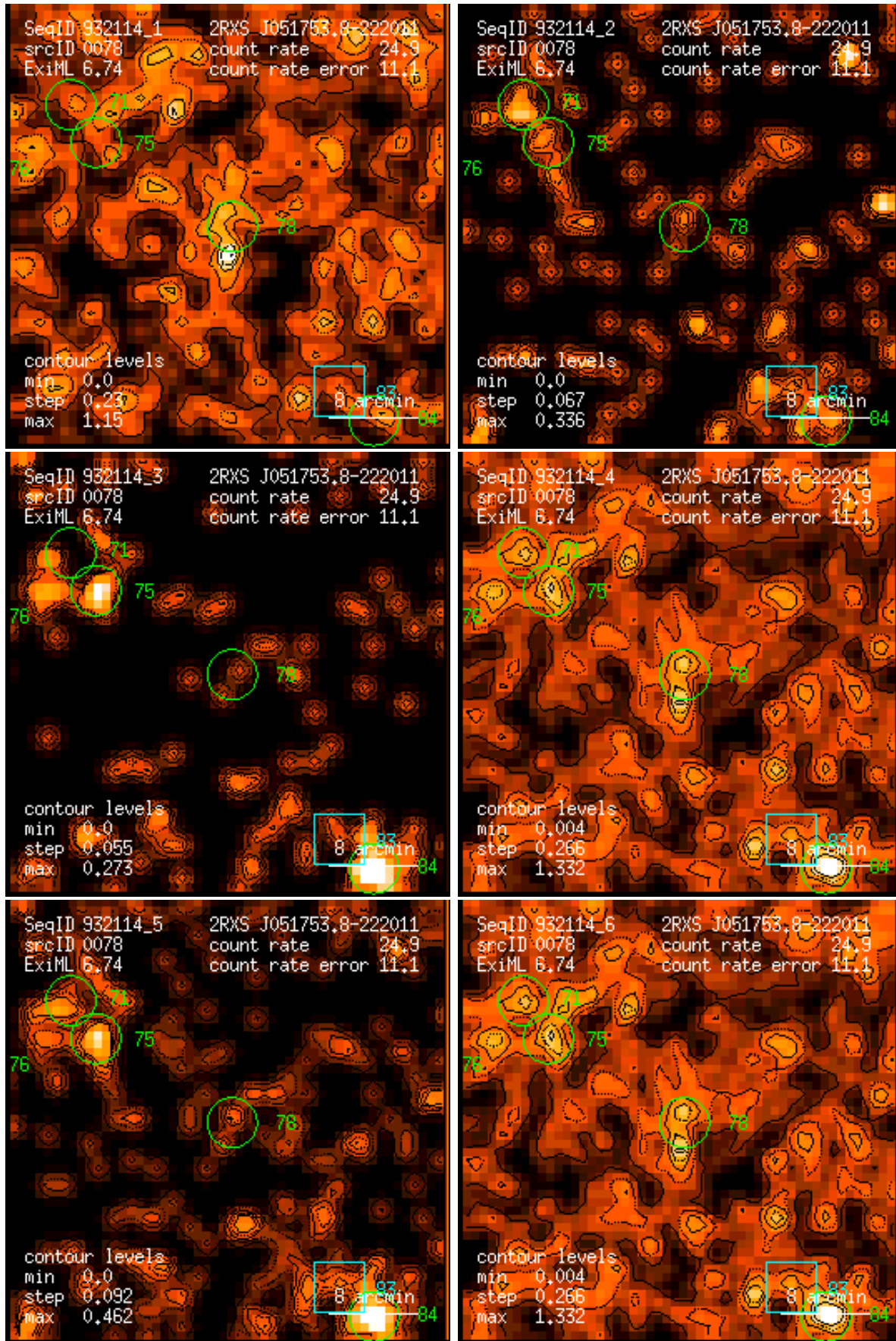
Figure 78: RASS 932114: detection 0078: band rate images, Gaussian filter: (1) PSPC channels 11 – 41, (2) 52 – 90, (3) 91 – 201, (4) 11 – 235, (5) 52 – 201, (6) 11 – 201. Broad band rates in counts/ks. Band rate contour levels in counts/ks/arcmin 2 .
