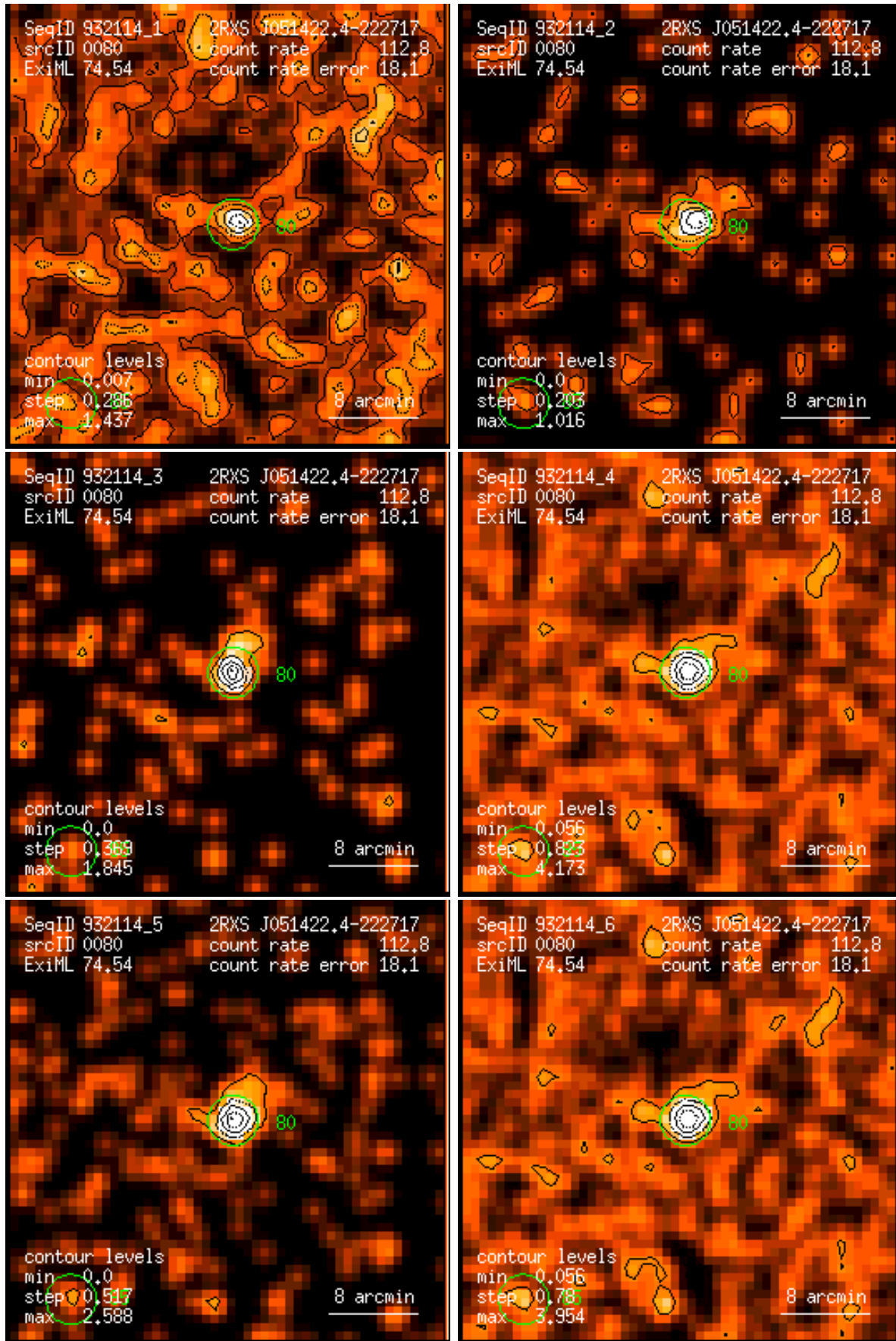
Figure 80: RASS 932114: detection 0080: band rate images, Gaussian filter: (1) PSPC channels 11 – 41, (2) 52 – 90, (3) 91 – 201, (4) 11 – 235, (5) 52 – 201, (6) 11 – 201. Broad band rates in counts/ks. Band rate contour levels in counts/ks/arcmin 2 .
