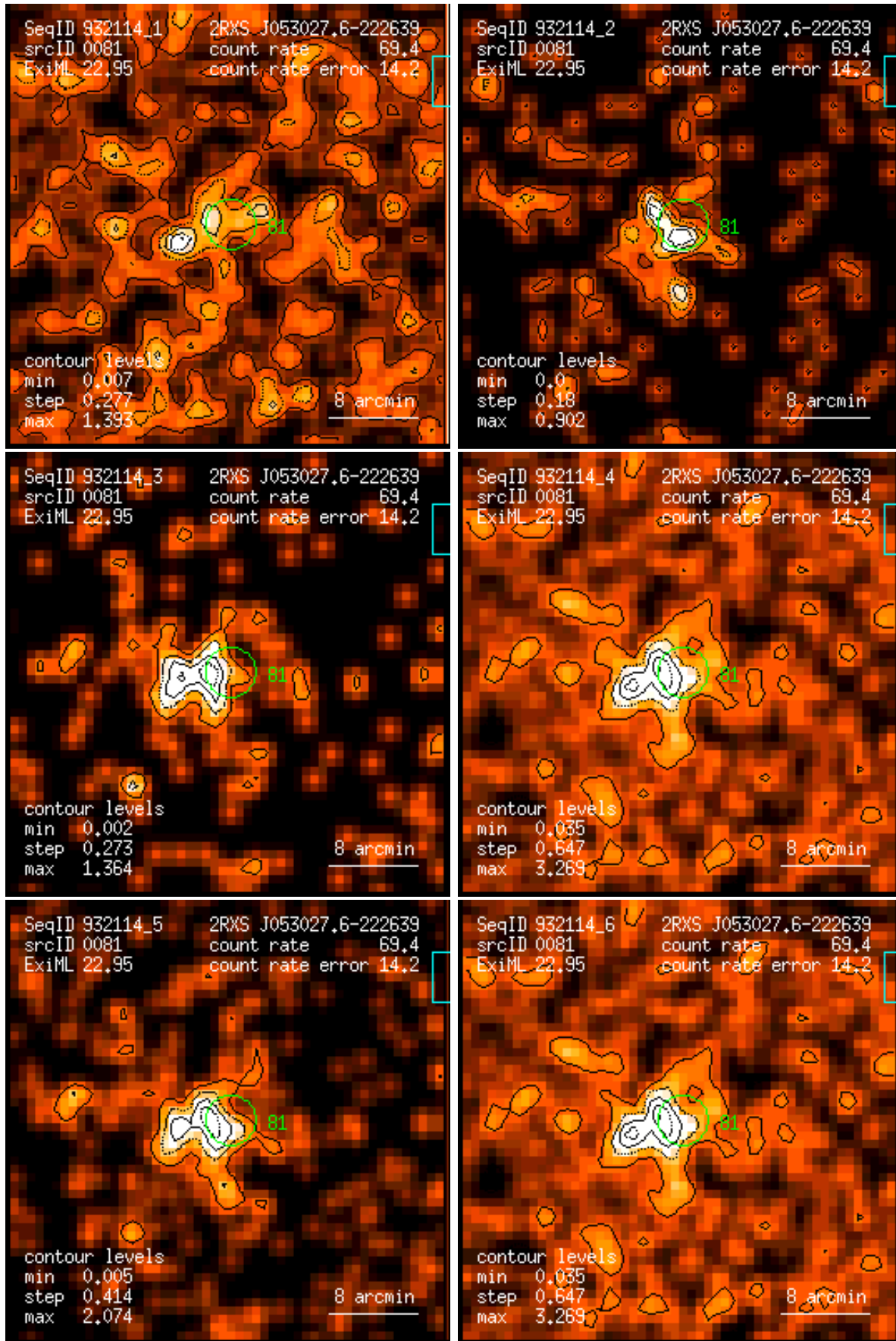
Figure 81: RASS 932114: detection 0081: band rate images, Gaussian filter: (1) PSPC channels 11 – 41, (2) 52 – 90, (3) 91 – 201, (4) 11 – 235, (5) 52 – 201, (6) 11 – 201. Broad band rates in counts/ks. Band rate contour levels in counts/ks/arcmin 2 .
