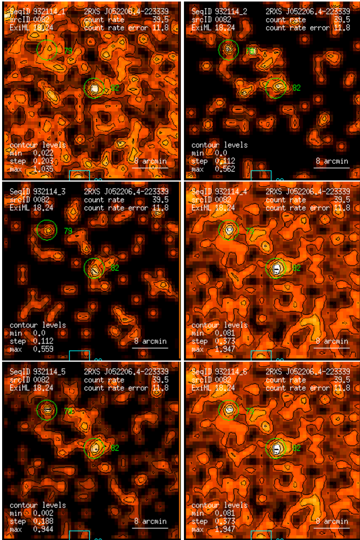
Figure 82: RASS 932114: detection 0082: band rate images, Gaussian filter: (1) PSPC channels 11 – 41, (2) 52 – 90, (3) 91 – 201, (4) 11 – 235, (5) 52 – 201, (6) 11 – 201. Broad band rates in counts/ks. Band rate contour levels in counts/ks/arcmin 2 .
