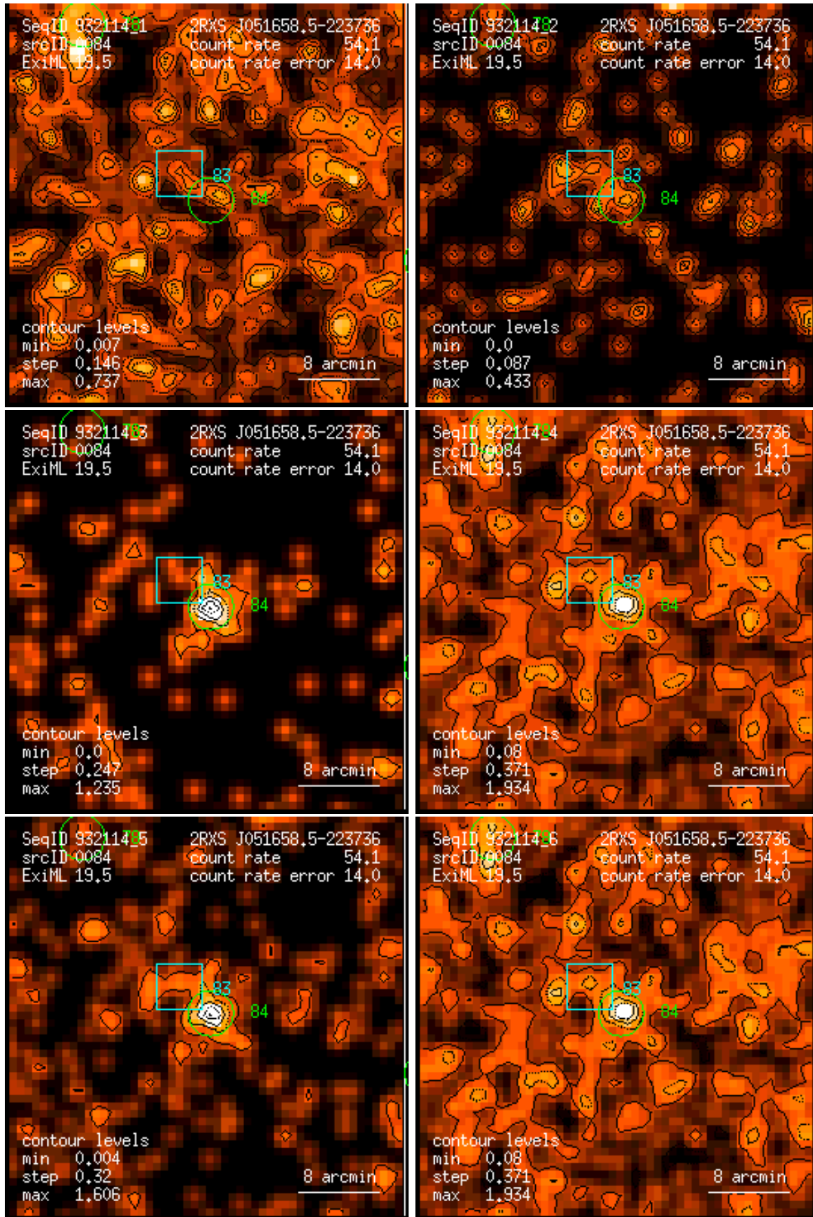
Figure 84: RASS 932114: detection 0084: band rate images, Gaussian filter: (1) PSPC channels 11 – 41, (2) 52 – 90, (3) 91 – 201, (4) 11 – 235, (5) 52 – 201, (6) 11 – 201. Broad band rates in counts/ks. Band rate contour levels in counts/ks/arcmin 2 .
