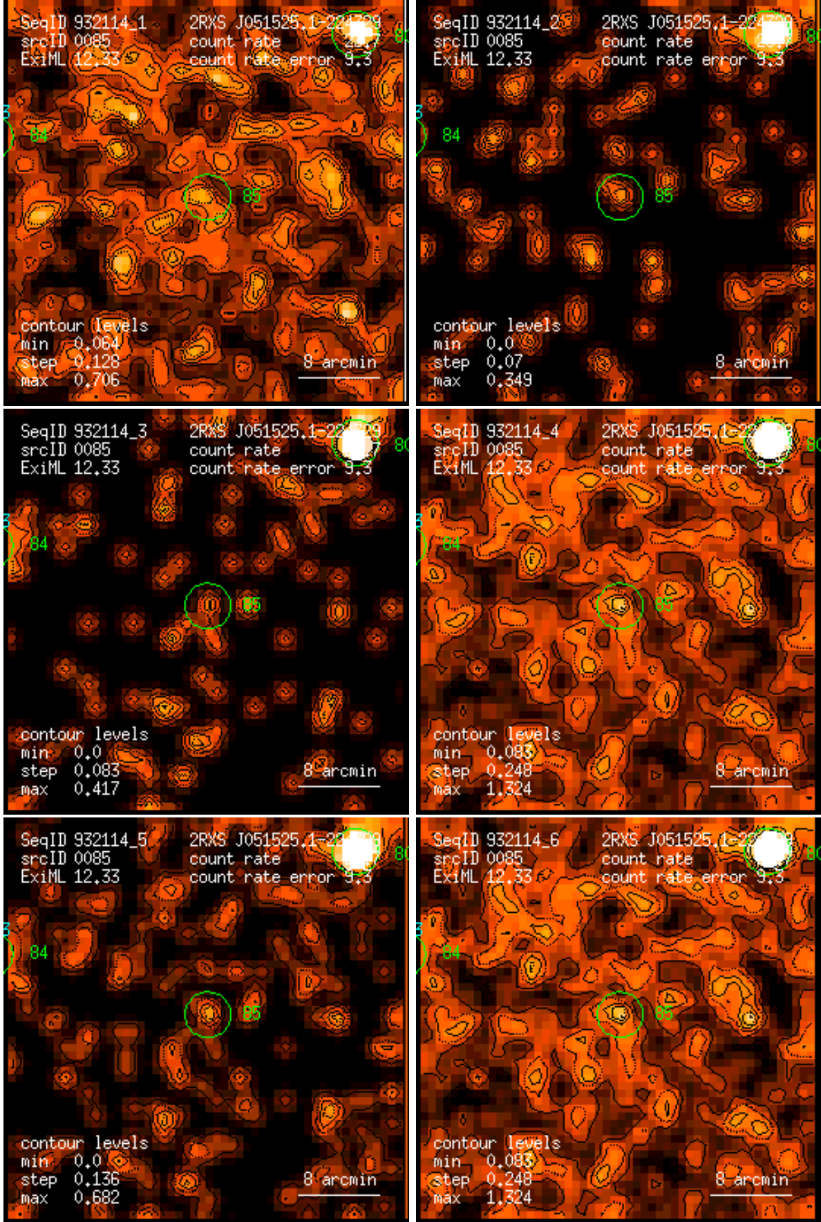
Figure 85: RASS 932114: detection 0085: band rate images, Gaussian filter: (1) PSPC channels 11 – 41, (2) 52 – 90, (3) 91 – 201, (4) 11 – 235, (5) 52 – 201, (6) 11 – 201. Broad band rates in counts/ks. Band rate contour levels in counts/ks/arcmin 2 .
