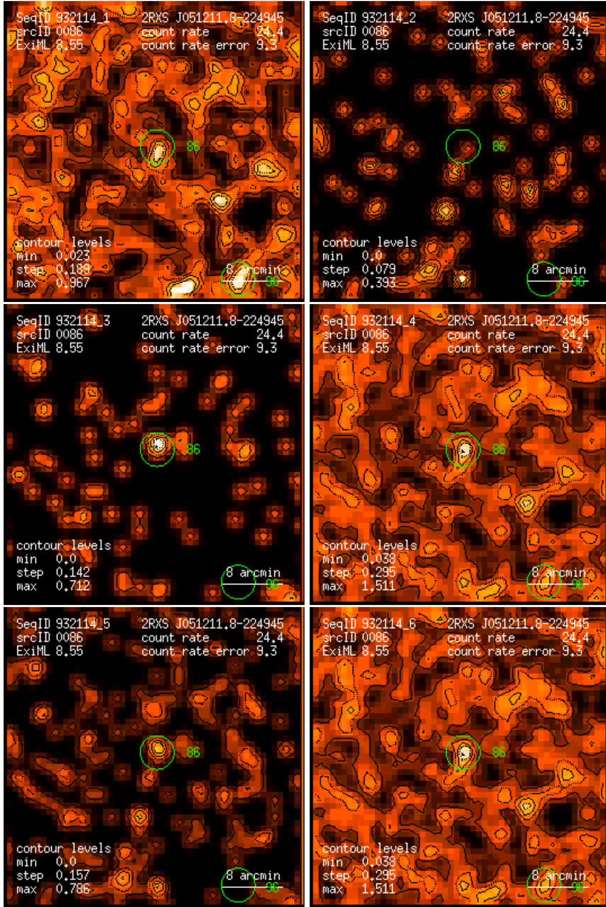
Figure 86: RASS 932114: detection 0086: band rate images, Gaussian filter: (1) PSPC channels 11 – 41, (2) 52 – 90, (3) 91 – 201, (4) 11 – 235, (5) 52 – 201, (6) 11 – 201. Broad band rates in counts/ks. Band rate contour levels in counts/ks/arcmin 2 .
