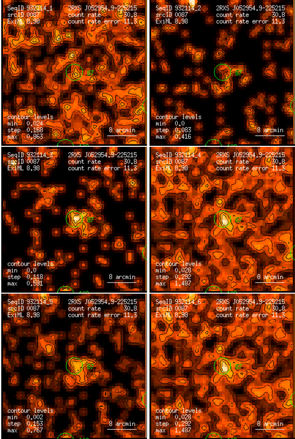
Figure 87: RASS 932114: detection 0087: band rate images, Gaussian filter: (1) PSPC channels 11 – 41, (2) 52 – 90, (3) 91 – 201, (4) 11 – 235, (5) 52 – 201, (6) 11 – 201. Broad band rates in counts/ks. Band rate contour levels in counts/ks/arcmin 2 .
