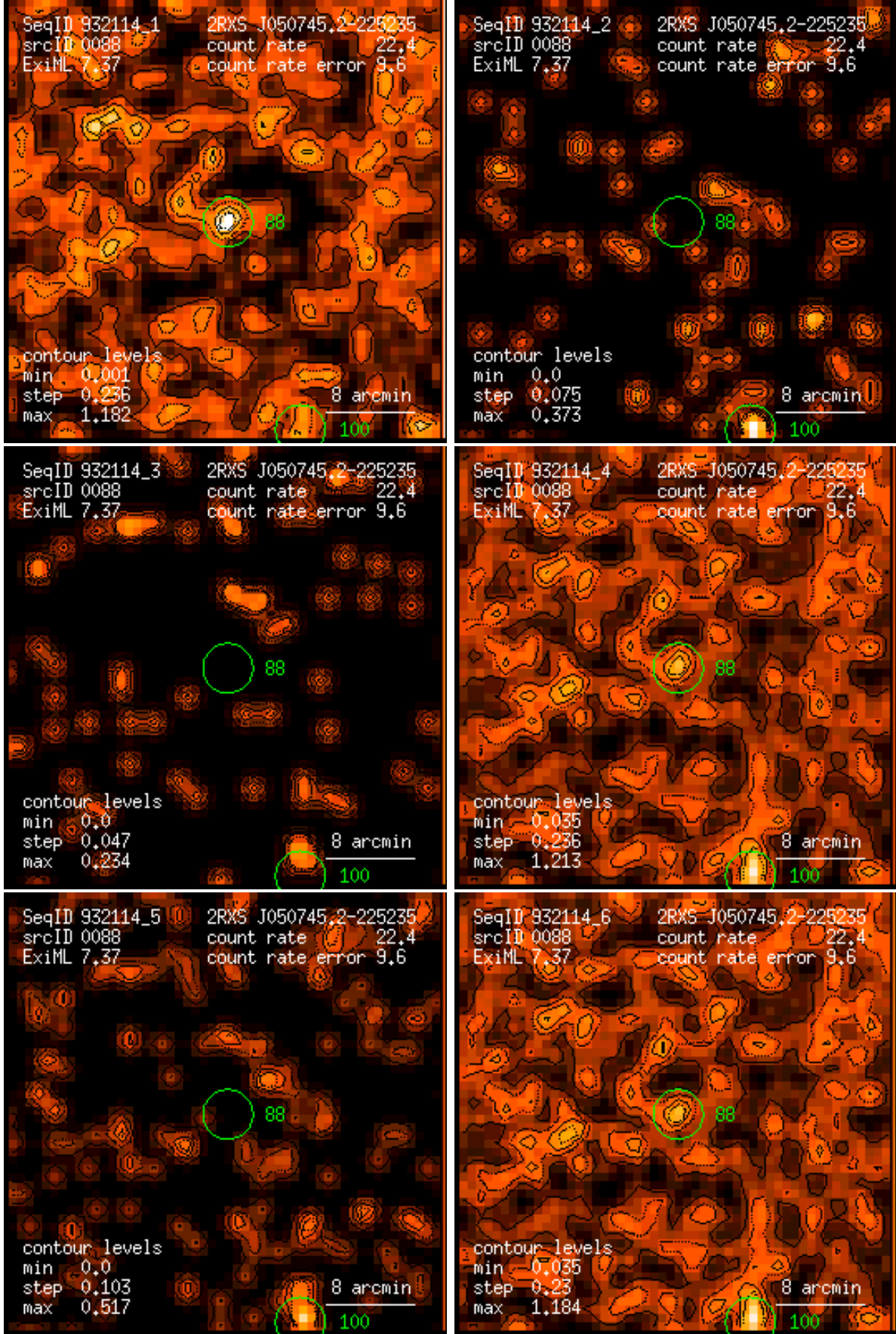
Figure 88: RASS 932114: detection 0088: band rate images, Gaussian filter: (1) PSPC channels 11 – 41, (2) 52 – 90, (3) 91 – 201, (4) 11 – 235, (5) 52 – 201, (6) 11 – 201. Broad band rates in counts/ks. Band rate contour levels in counts/ks/arcmin 2 .
