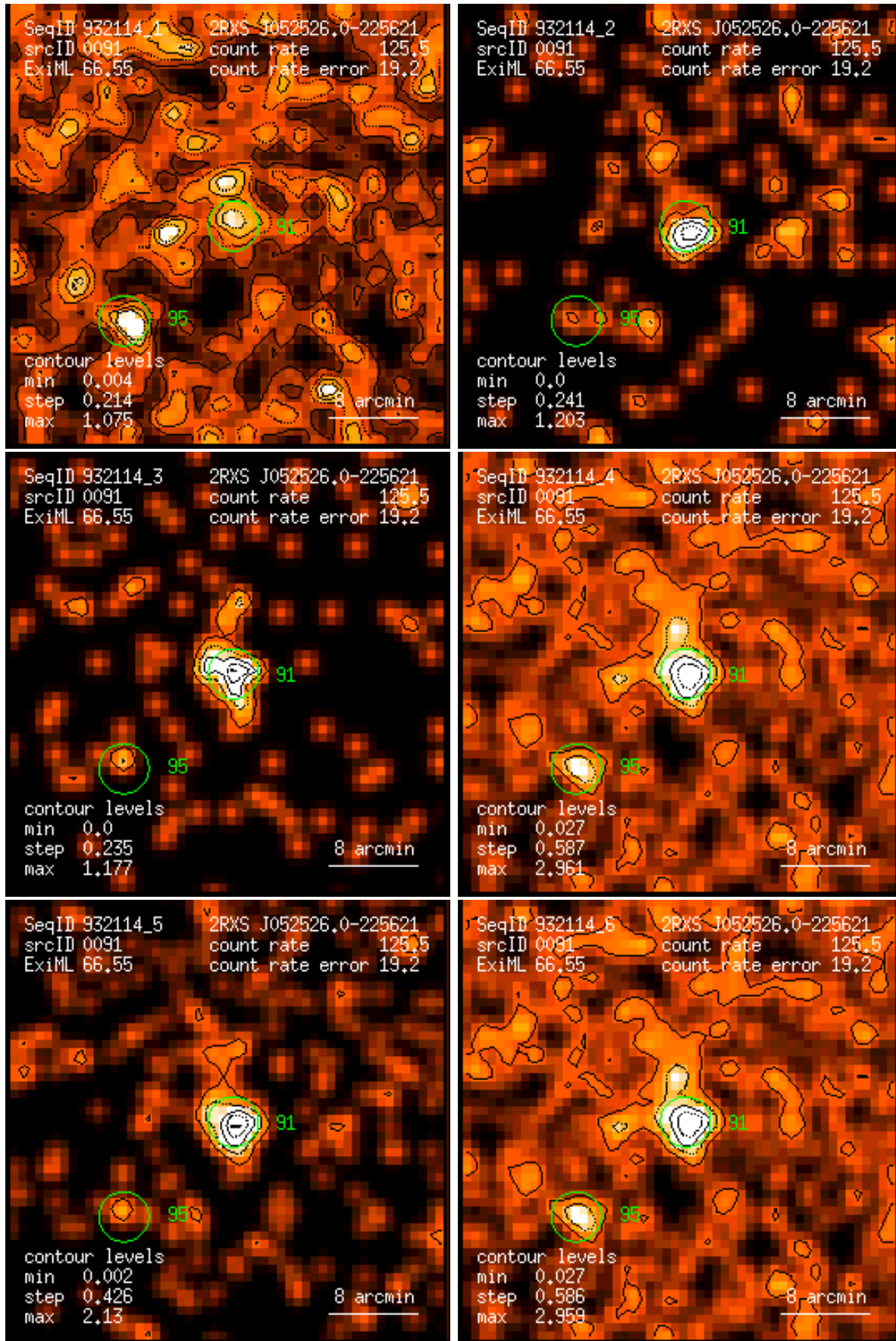
Figure 91: RASS 932114: detection 0091: band rate images, Gaussian filter: (1) PSPC channels 11 – 41, (2) 52 – 90, (3) 91 – 201, (4) 11 – 235, (5) 52 – 201, (6) 11 – 201. Broad band rates in counts/ks. Band rate contour levels in counts/ks/arcmin 2 .
