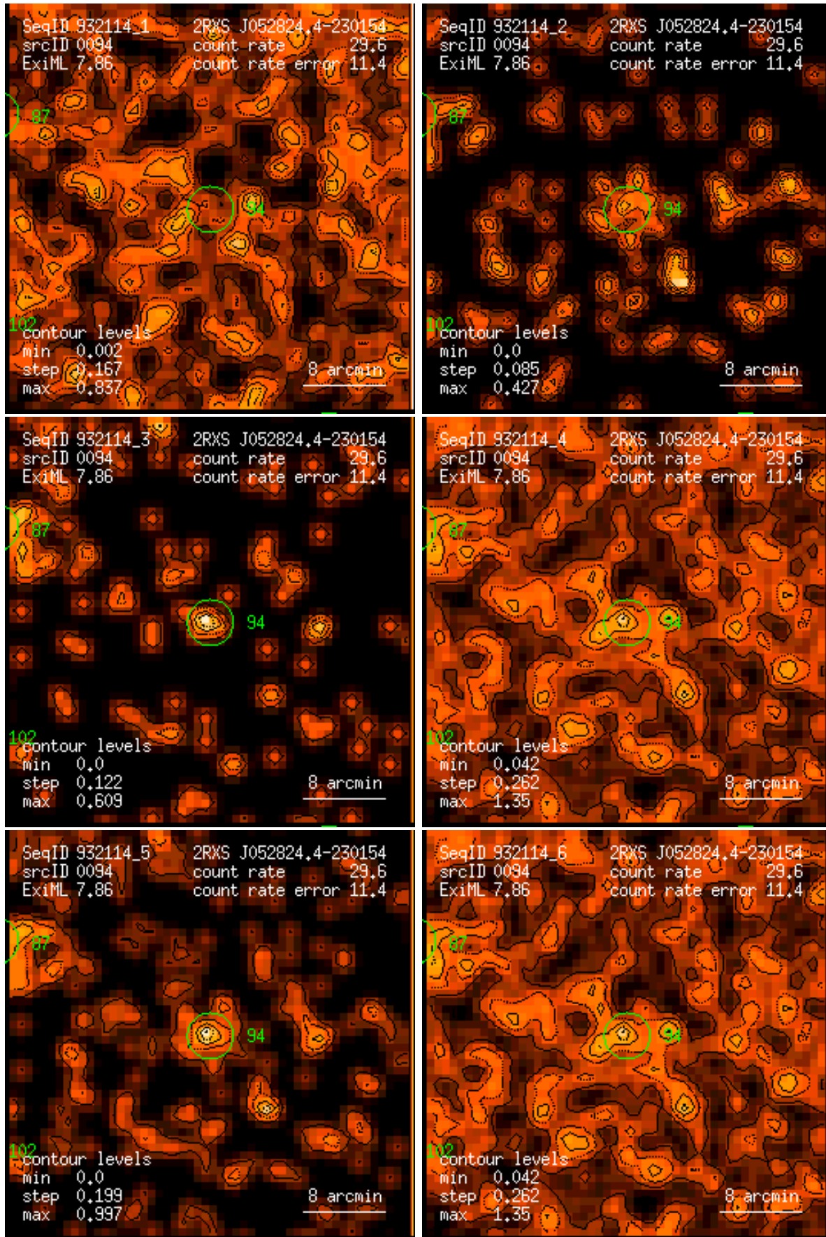
Figure 94: RASS 932114: detection 0094: band rate images, Gaussian filter: (1) PSPC channels 11 – 41, (2) 52 – 90, (3) 91 – 201, (4) 11 – 235, (5) 52 – 201, (6) 11 – 201. Broad band rates in counts/ks. Band rate contour levels in counts/ks/arcmin 2 .
