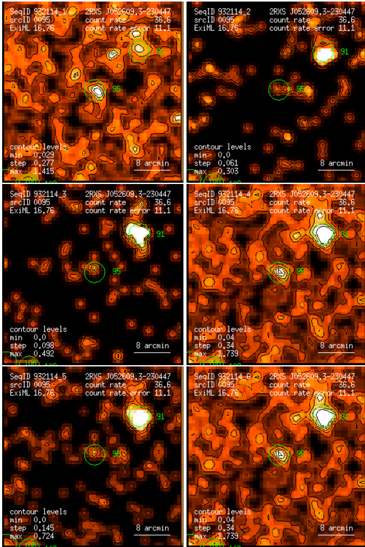
Figure 95: RASS 932114: detection 0095: band rate images, Gaussian filter: (1) PSPC channels 11 – 41, (2) 52 – 90, (3) 91 – 201, (4) 11 – 235, (5) 52 – 201, (6) 11 – 201. Broad band rates in counts/ks. Band rate contour levels in counts/ks/arcmin 2 .
