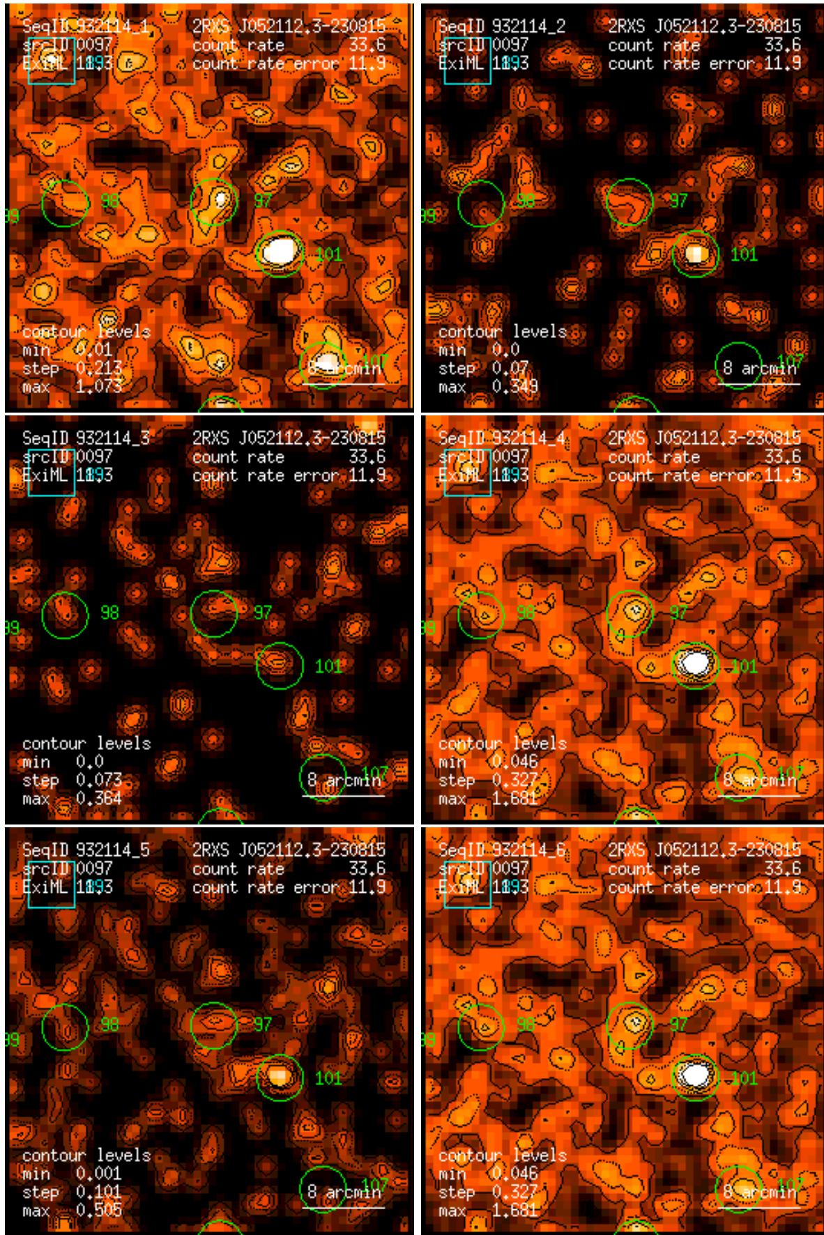
Figure 97: RASS 932114: detection 0097: band rate images, Gaussian filter: (1) PSPC channels 11 – 41, (2) 52 – 90, (3) 91 – 201, (4) 11 – 235, (5) 52 – 201, (6) 11 – 201. Broad band rates in counts/ks. Band rate contour levels in counts/ks/arcmin 2 .
