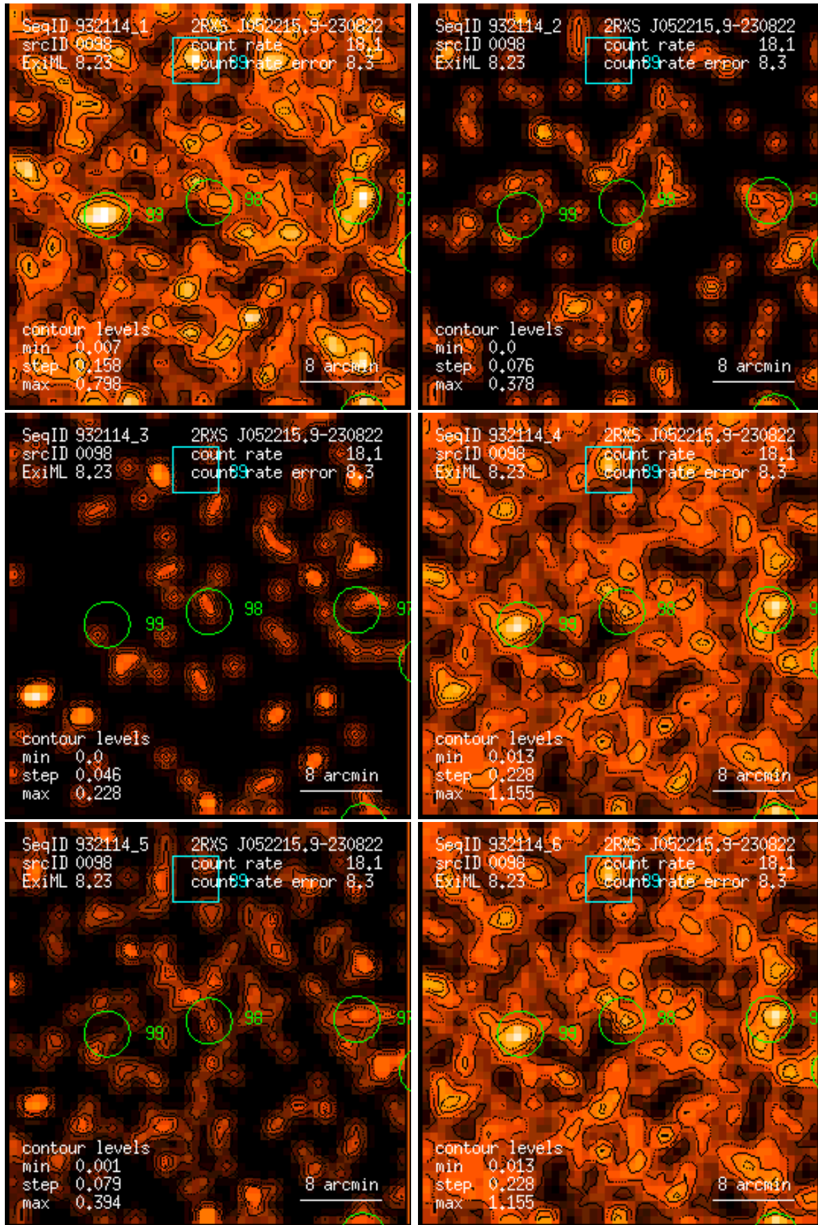
Figure 98: RASS 932114: detection 0098: band rate images, Gaussian filter: (1) PSPC channels 11 – 41, (2) 52 – 90, (3) 91 – 201, (4) 11 – 235, (5) 52 – 201, (6) 11 – 201. Broad band rates in counts/ks. Band rate contour levels in counts/ks/arcmin 2 .
