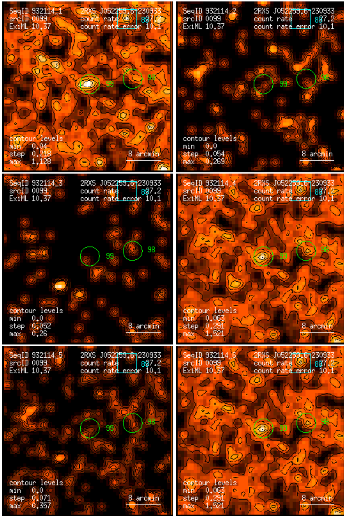
Figure 99: RASS 932114: detection 0099: band rate images, Gaussian filter: (1) PSPC channels 11 – 41, (2) 52 – 90, (3) 91 – 201, (4) 11 – 235, (5) 52 – 201, (6) 11 – 201. Broad band rates in counts/ks. Band rate contour levels in counts/ks/arcmin 2 .
