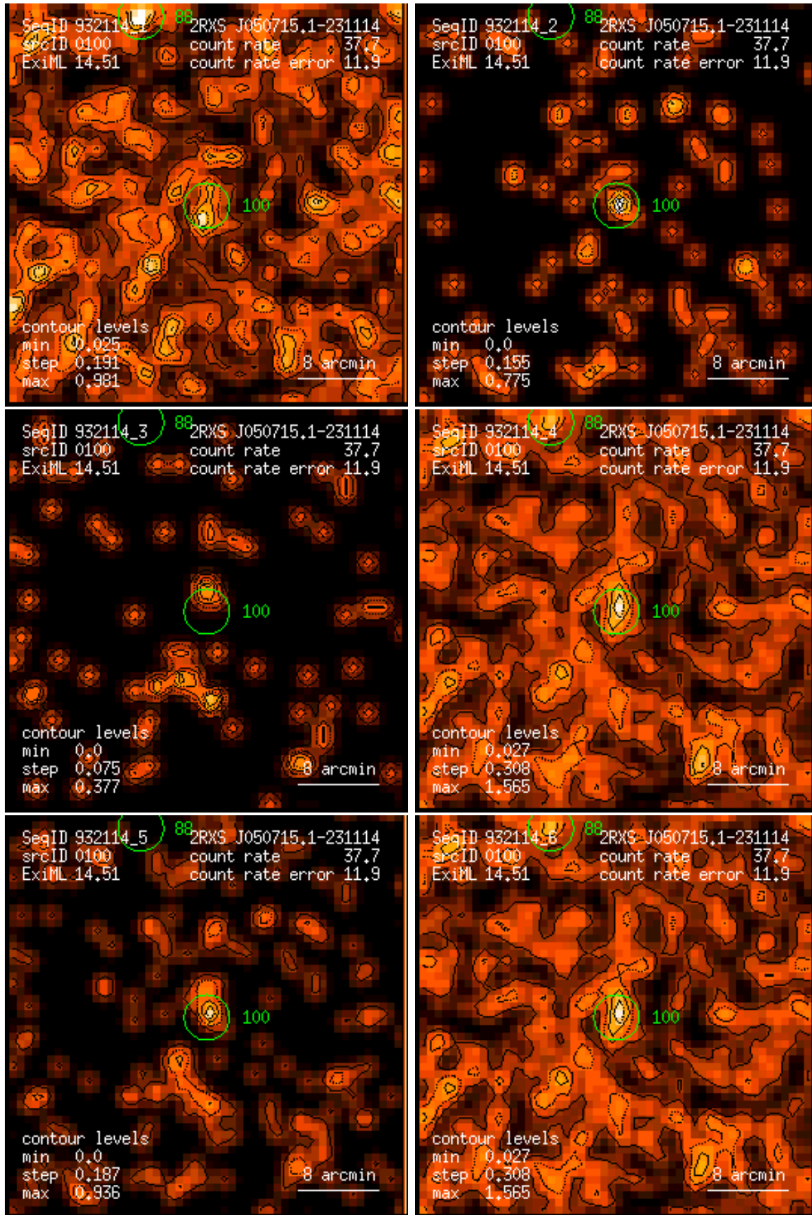
Figure 100: RASS 932114: detection 0100: band rate images, Gaussian filter: (1) PSPC channels 11 – 41, (2) 52 – 90, (3) 91 – 201, (4) 11 – 235, (5) 52 – 201, (6) 11 – 201. Broad band rates in counts/ks. Band rate contour levels in counts/ks/arcmin 2 .
