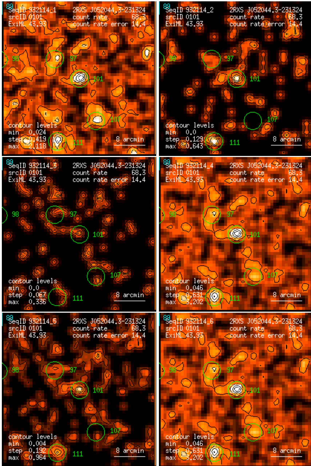
Figure 101: RASS 932114: detection 0101: band rate images, Gaussian filter: (1) PSPC channels 11 – 41, (2) 52 – 90, (3) 91 – 201, (4) 11 – 235, (5) 52 – 201, (6) 11 – 201. Broad band rates in counts/ks. Band rate contour levels in counts/ks/arcmin 2 .
