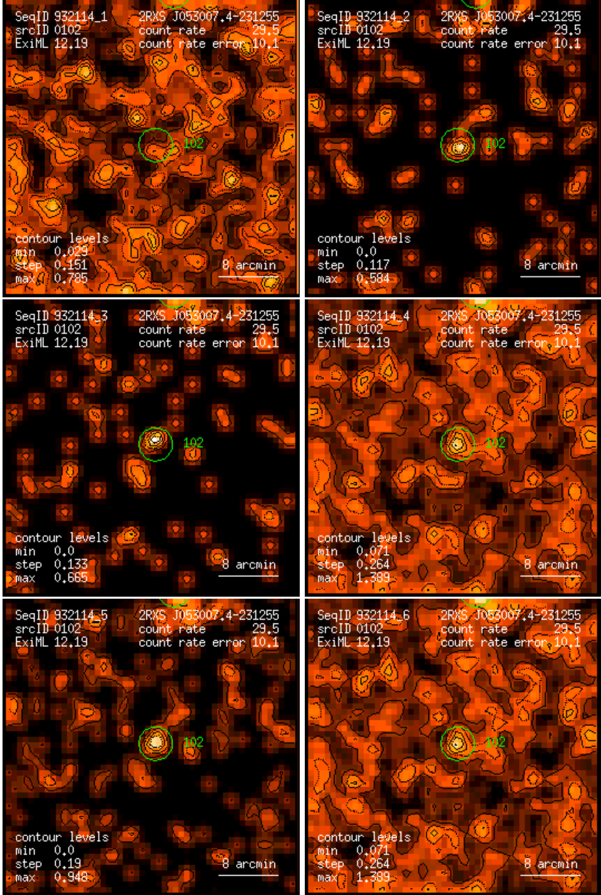
Figure 102: RASS 932114: detection 0102: band rate images, Gaussian filter: (1) PSPC channels 11 – 41, (2) 52 – 90, (3) 91 – 201, (4) 11 – 235, (5) 52 – 201, (6) 11 – 201. Broad band rates in counts/ks. Band rate contour levels in counts/ks/arcmin 2 .
