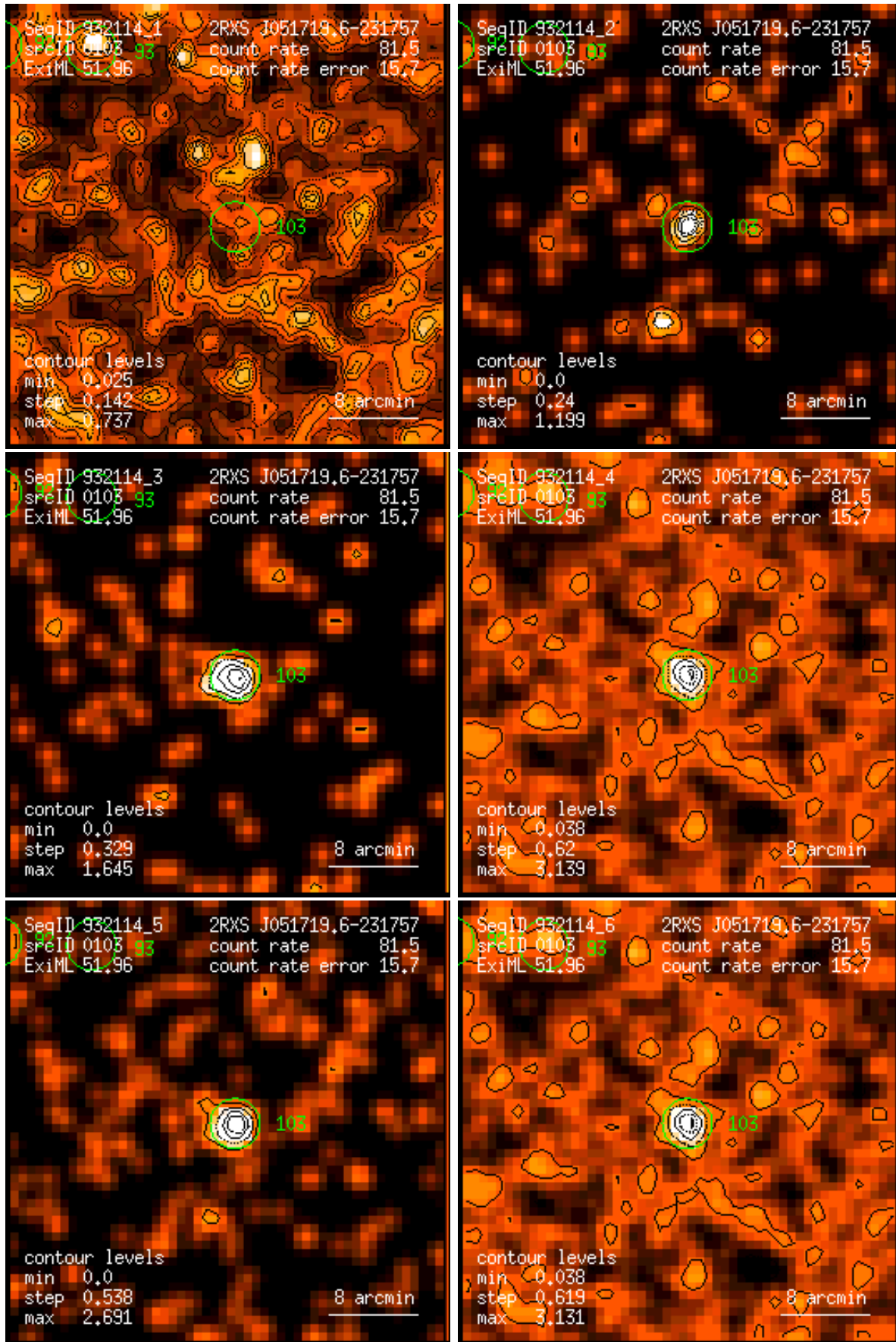
Figure 103: RASS 932114: detection 0103: band rate images, Gaussian filter: (1) PSPC channels 11 – 41, (2) 52 – 90, (3) 91 – 201, (4) 11 – 235, (5) 52 – 201, (6) 11 – 201. Broad band rates in counts/ks. Band rate contour levels in counts/ks/arcmin 2 .
