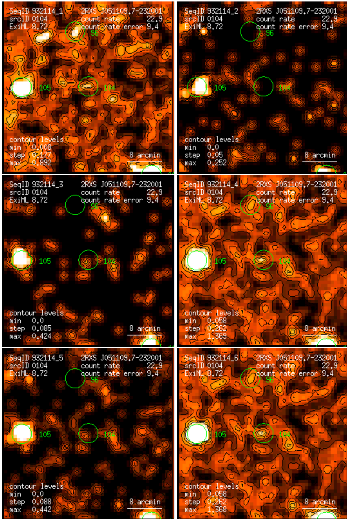
Figure 104: RASS 932114: detection 0104: band rate images, Gaussian filter: (1) PSPC channels 11 – 41, (2) 52 – 90, (3) 91 – 201, (4) 11 – 235, (5) 52 – 201, (6) 11 – 201. Broad band rates in counts/ks. Band rate contour levels in counts/ks/arcmin 2 .
