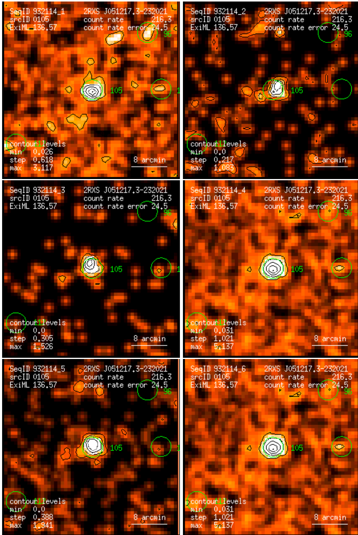
Figure 105: RASS 932114: detection 0105: band rate images, Gaussian filter: (1) PSPC channels 11 – 41, (2) 52 – 90, (3) 91 – 201, (4) 11 – 235, (5) 52 – 201, (6) 11 – 201. Broad band rates in counts/ks. Band rate contour levels in counts/ks/arcmin 2 .
