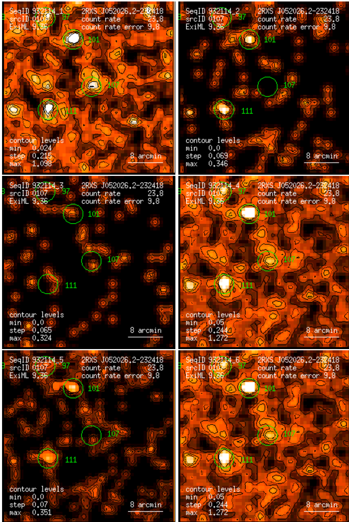
Figure 107: RASS 932114: detection 0107: band rate images, Gaussian filter: (1) PSPPC channels 11 – 41, (2) 52 – 90, (3) 91 – 201, (4) 11 – 235, (5) 52 – 201, (6) 11 – 201. Broad band rates in counts/ks. Band rate contour levels in counts/ks/arcmin 2 .
