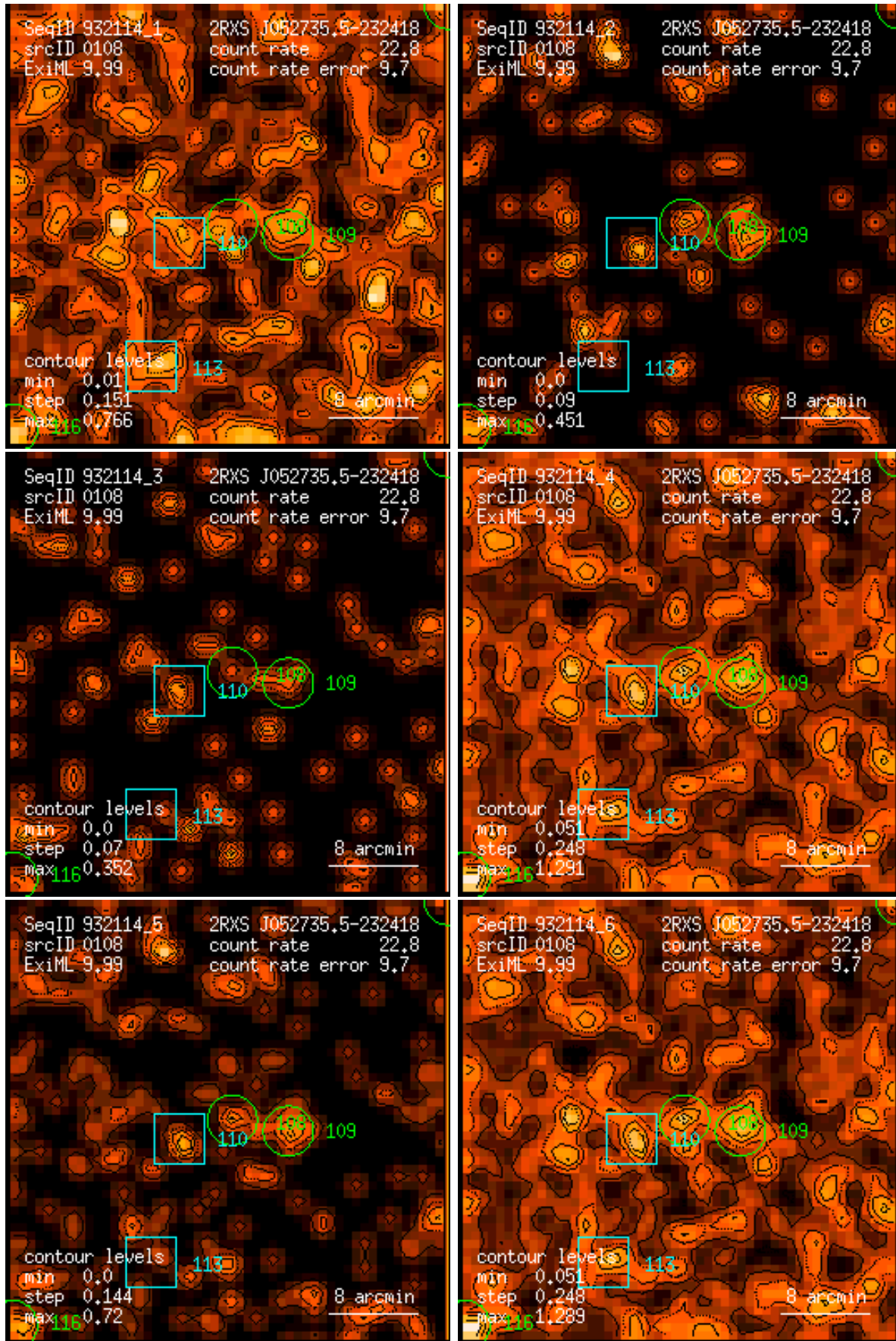
Figure 108: RASS 932114: detection 0108: band rate images, Gaussian filter: (1) PSPC channels 11 – 41, (2) 52 – 90, (3) 91 – 201, (4) 11 – 235, (5) 52 – 201, (6) 11 – 201. Broad band rates in counts/ks. Band rate contour levels in counts/ks/arcmin 2 .
