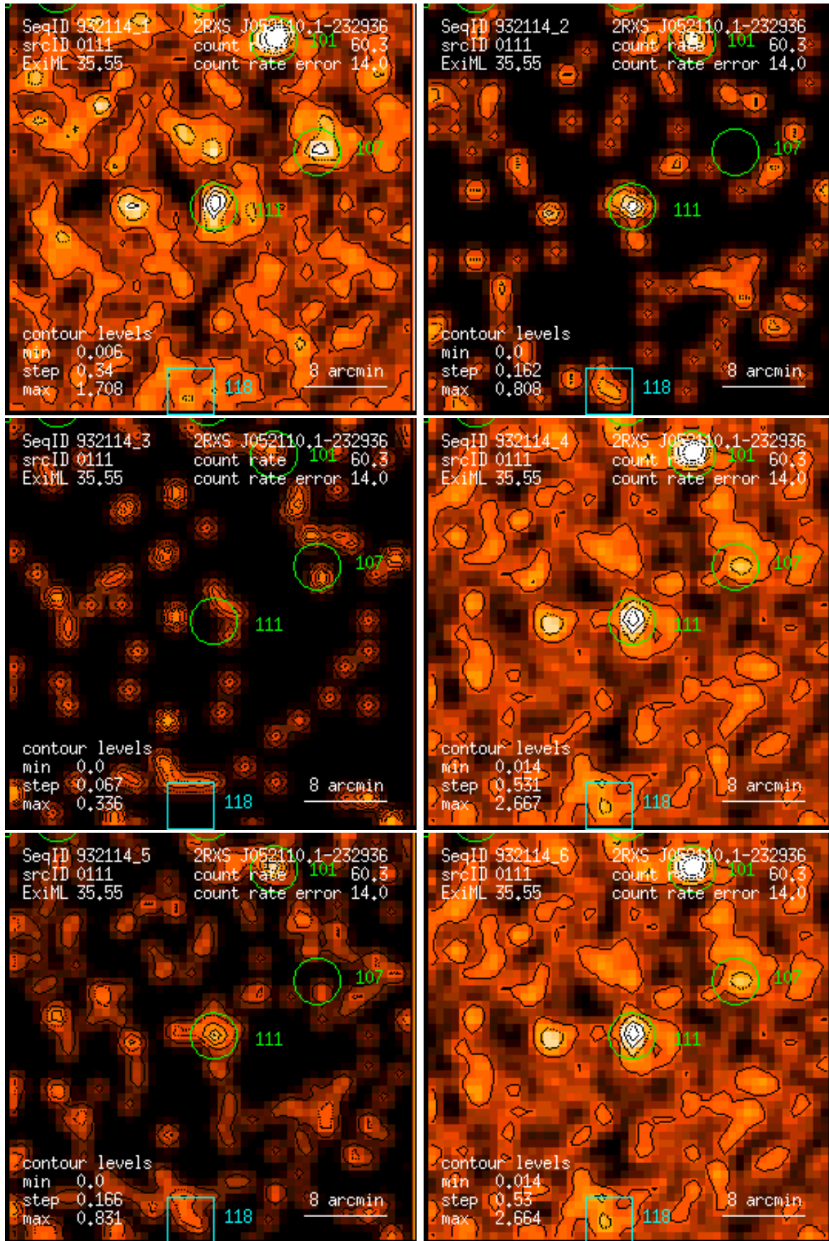
Figure 111: RASS 932114: detection 0111: band rate images, Gaussian filter: (1) PSPC channels 11 – 41, (2) 52 – 90, (3) 91 – 201, (4) 11 – 235, (5) 52 – 201, (6) 11 – 201. Broad band rates in counts/ks. Band rate contour levels in counts/ks/arcmin 2 .
