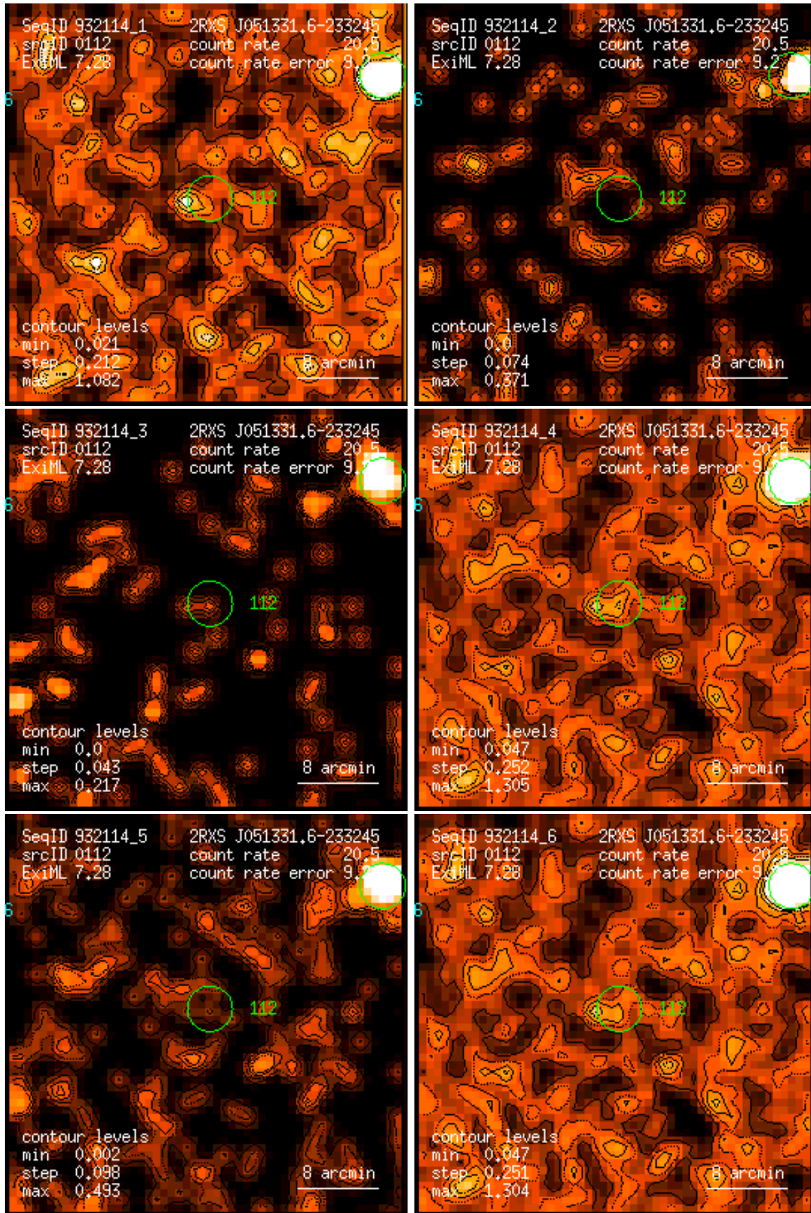
Figure 112: RASS 932114: detection 0112: band rate images, Gaussian filter: (1) PSPC channels 11 – 41, (2) 52 – 90, (3) 91 – 201, (4) 11 – 235, (5) 52 – 201, (6) 11 – 201. Broad band rates in counts/ks. Band rate contour levels in counts/ks/arcmin 2 .
