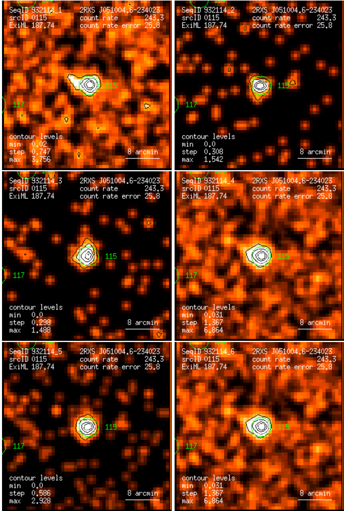
Figure 115: RASS 932114: detection 0115: band rate images, Gaussian filter: (1) PSPC channels 11 – 41, (2) 52 – 90, (3) 91 – 201, (4) 11 – 235, (5) 52 – 201, (6) 11 – 201. Broad band rates in counts/ks. Band rate contour levels in counts/ks/arcmin 2 .
