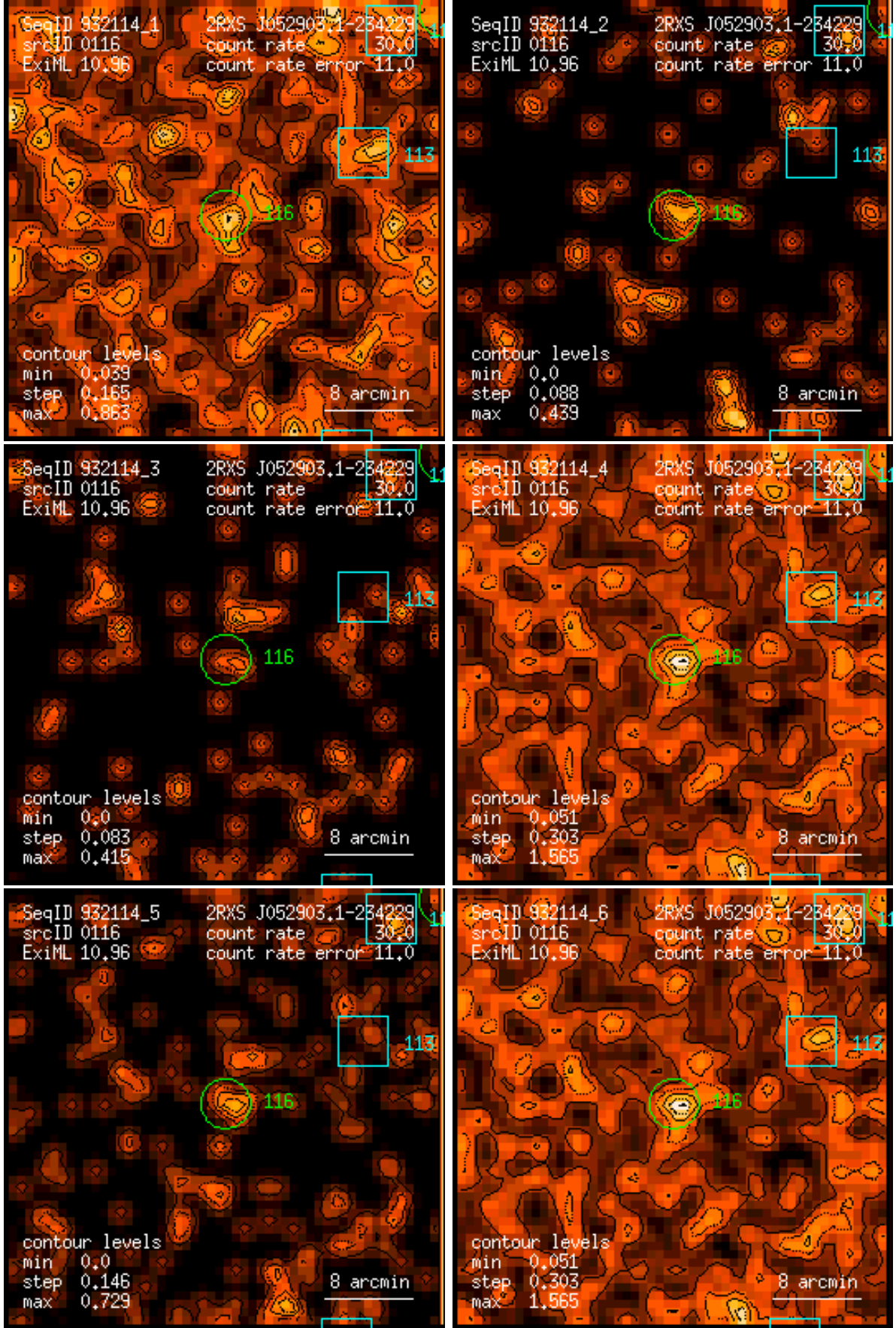
Figure 116: RASS 932114: detection 0116: band rate images, Gaussian filter: (1) PSPC channels 11 – 41, (2) 52 – 90, (3) 91 – 201, (4) 11 – 235, (5) 52 – 201, (6) 11 – 201. Broad band rates in counts/ks. Band rate contour levels in counts/ks/arcmin 2 .
