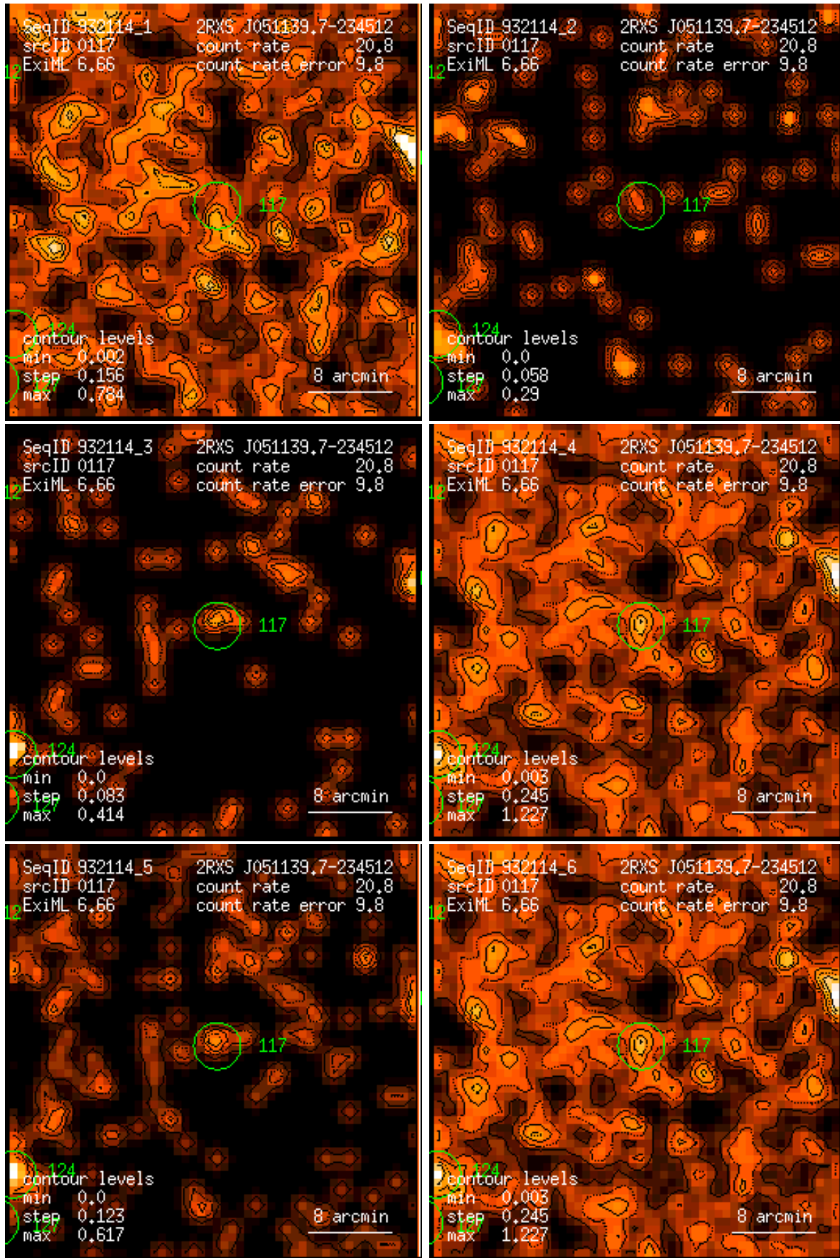
Figure 117: RASS 932114: detection 0117: band rate images, Gaussian filter: (1) PSPC channels 11 – 41, (2) 52 – 90, (3) 91 – 201, (4) 11 – 235, (5) 52 – 201, (6) 11 – 201. Broad band rates in counts/ks. Band rate contour levels in counts/ks/arcmin 2 .
