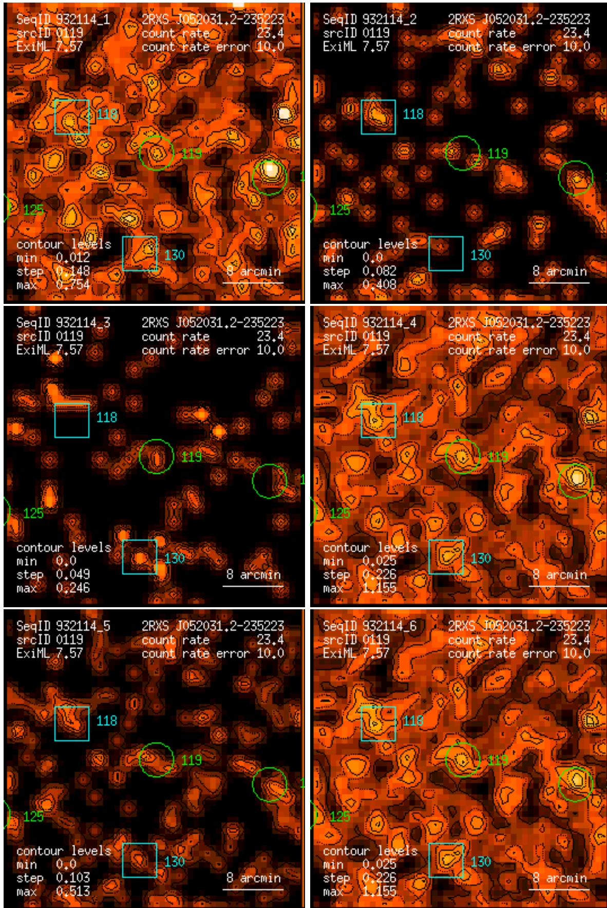
Figure 119: RASS 932114: detection 0119: band rate images, Gaussian filter: (1) PSPC channels 11 – 41, (2) 52 – 90, (3) 91 – 201, (4) 11 – 235, (5) 52 – 201, (6) 11 – 201. Broad band rates in counts/ks. Band rate contour levels in counts/ks/arcmin 2 .
