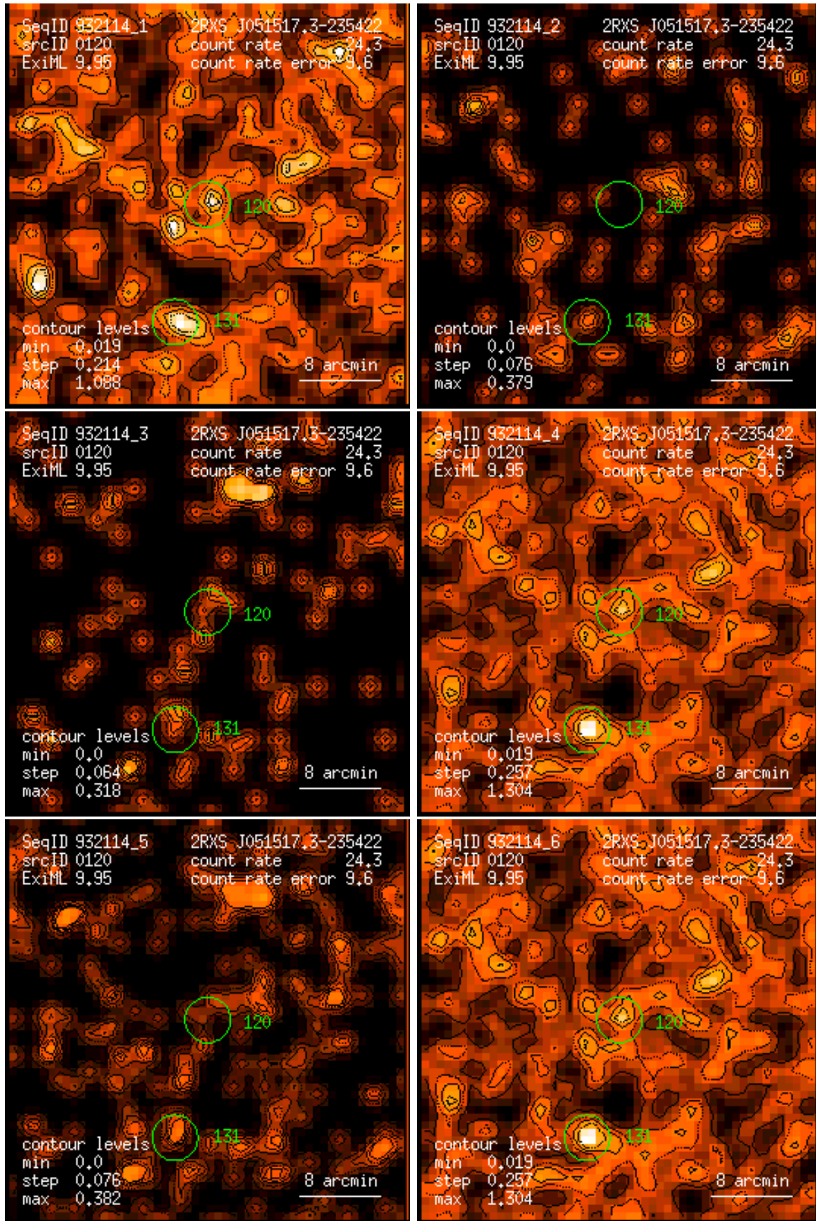
Figure 120: RASS 932114: detection 0120: band rate images, Gaussian filter: (1) PSPC channels 11 – 41, (2) 52 – 90, (3) 91 – 201, (4) 11 – 235, (5) 52 – 201, (6) 11 – 201. Broad band rates in counts/ks. Band rate contour levels in counts/ks/arcmin 2 .
