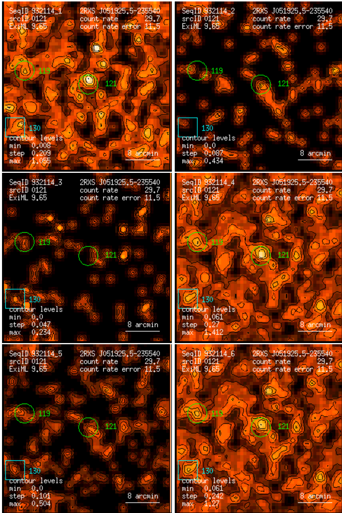
Figure 121: RASS 932114: detection 0121: band rate images, Gaussian filter: (1) PSPC channels 11 – 41, (2) 52 – 90, (3) 91 – 201, (4) 11 – 235, (5) 52 – 201, (6) 11 – 201. Broad band rates in counts/ks. Band rate contour levels in counts/ks/arcmin 2 .
