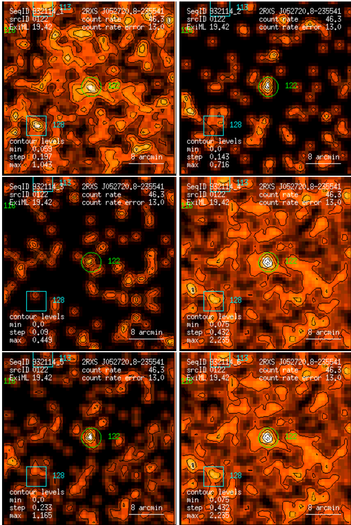
Figure 122: RASS 932114: detection 0122: band rate images, Gaussian filter: (1) PSPC channels 11 – 41, (2) 52 – 90, (3) 91 – 201, (4) 11 – 235, (5) 52 – 201, (6) 11 – 201. Broad band rates in counts/ks. Band rate contour levels in counts/ks/arcmin 2 .
