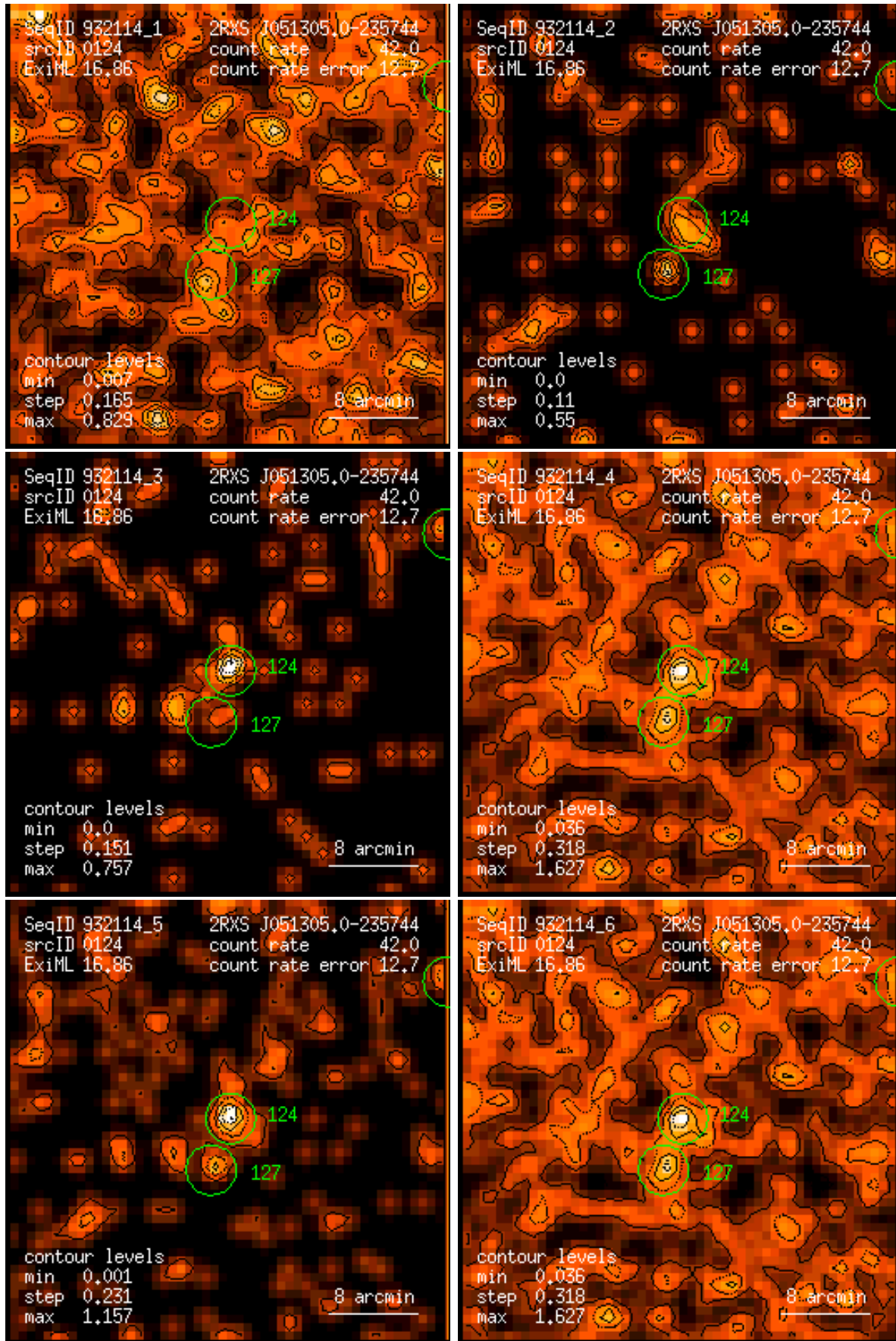
Figure 124: RASS 932114: detection 0124: band rate images, Gaussian filter: (1) PSPC channels 11 – 41, (2) 52 – 90, (3) 91 – 201, (4) 11 – 235, (5) 52 – 201, (6) 11 – 201. Broad band rates in counts/ks. Band rate contour levels in counts/ks/arcmin 2 .
