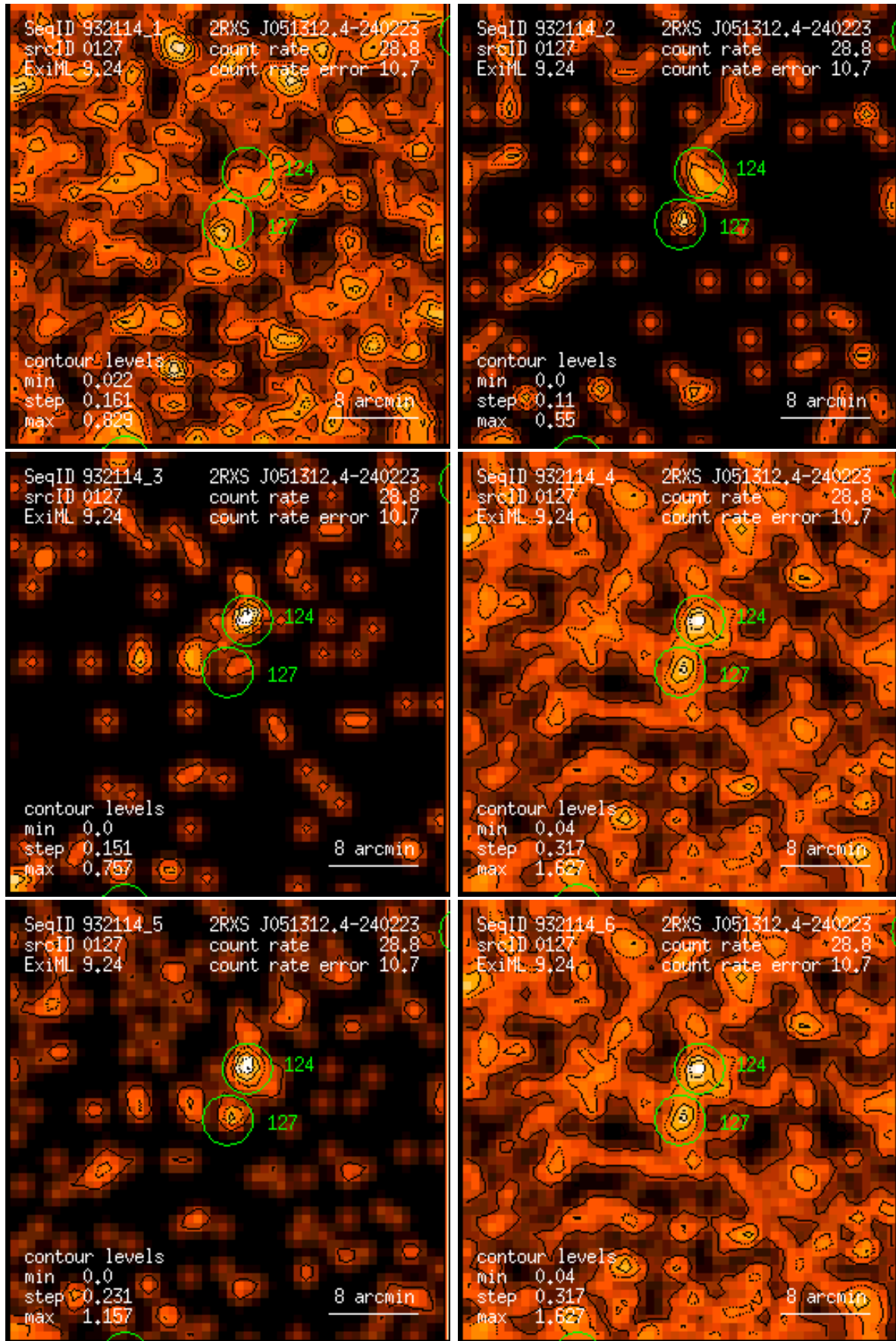
Figure 127: RASS 932114: detection 0127: band rate images, Gaussian filter: (1) PSPC channels 11 – 41, (2) 52 – 90, (3) 91 – 201, (4) 11 – 235, (5) 52 – 201, (6) 11 – 201. Broad band rates in counts/ks. Band rate contour levels in counts/ks/arcmin 2 .
