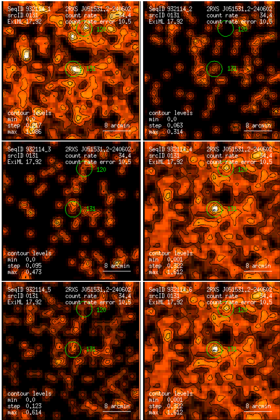
Figure 131: RASS 932114: detection 0131: band rate images, Gaussian filter: (1) PSPC channels 11 – 41, (2) 52 – 90, (3) 91 – 201, (4) 11 – 235, (5) 52 – 201, (6) 11 – 201. Broad band rates in counts/ks. Band rate contour levels in counts/ks/arcmin 2 .
