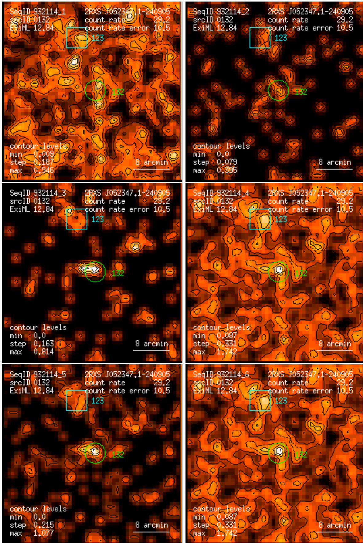
Figure 132: RASS 932114: detection 0132: band rate images, Gaussian filter: (1) PSPC channels 11 – 41, (2) 52 – 90, (3) 91 – 201, (4) 11 – 235, (5) 52 – 201, (6) 11 – 201. Broad band rates in counts/ks. Band rate contour levels in counts/ks/arcmin 2 .
