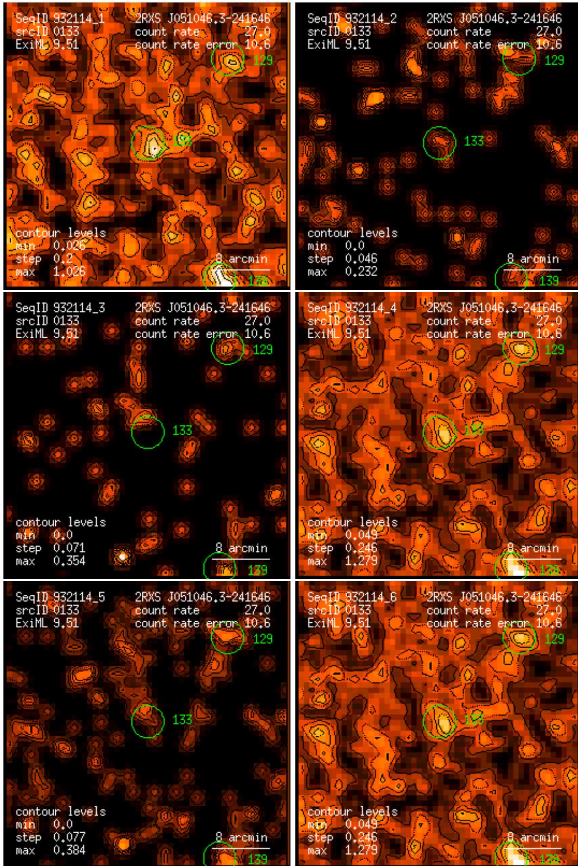
Figure 133: RASS 932114: detection 0133: band rate images, Gaussian filter: (1) PSPC channels 11 – 41, (2) 52 – 90, (3) 91 – 201, (4) 11 – 235, (5) 52 – 201, (6) 11 – 201. Broad band rates in counts/ks. Band rate contour levels in counts/ks/arcmin 2 .
